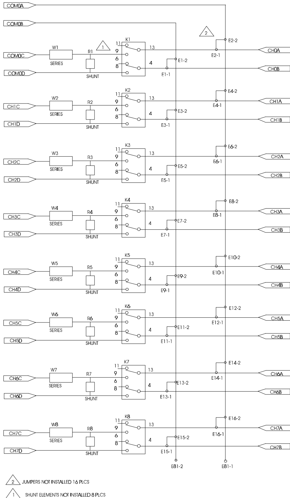
Figure 3-5, 1260-13 Jumper Locations
