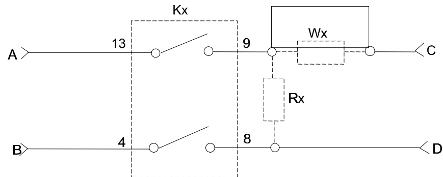
Figure 3-3, 1260-13 Channel
