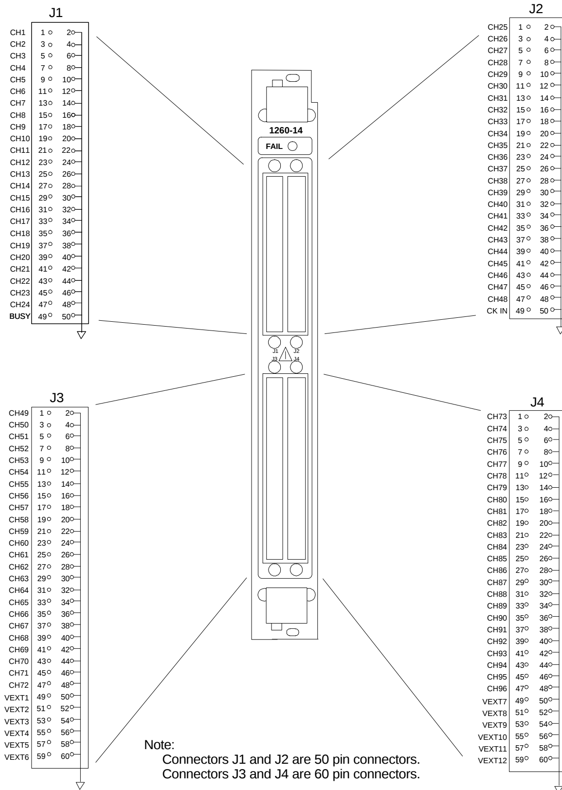
Figure 1-2, Model 1260-14C Front Panel and Pin Configuration
