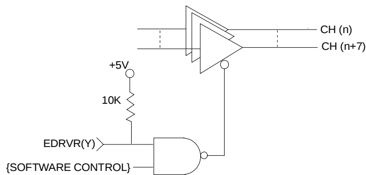
Figure 3-2, 1260-14 Tri-State Control
