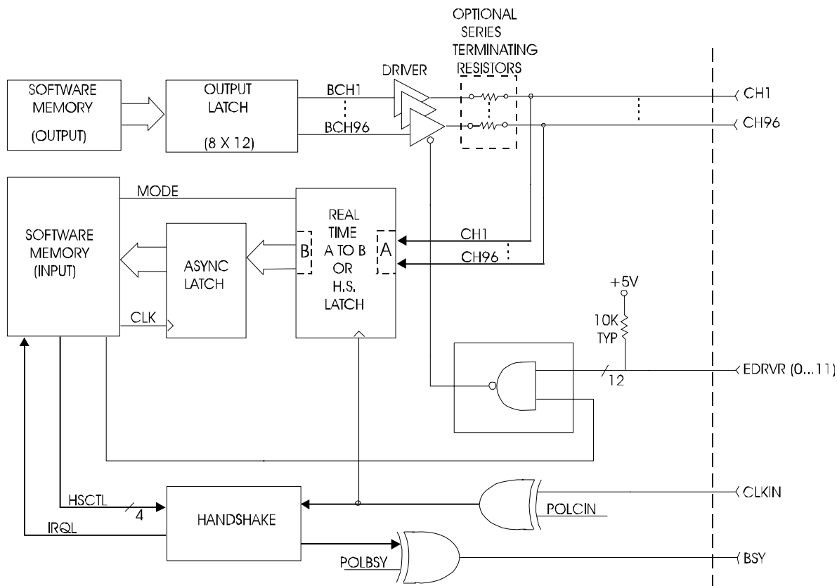
Figure 1-1, 1260-14 Block Diagram
