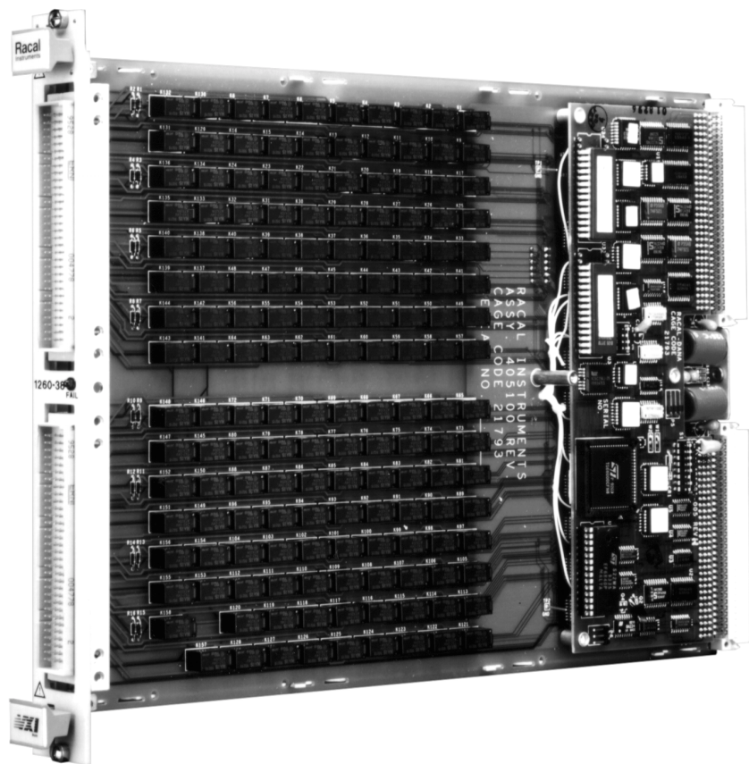
Figure 1-1, 1260-38 Multiplexer / Scanner
