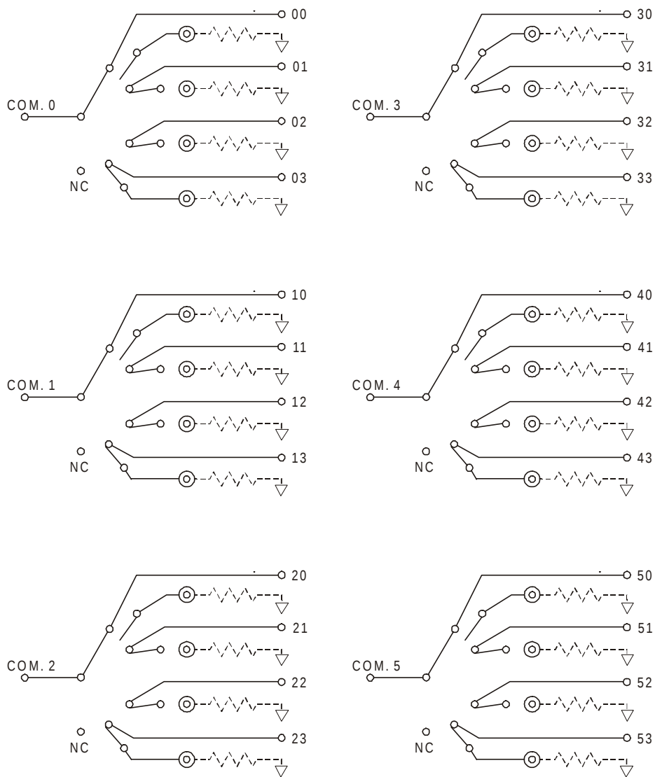
Figure 1-2, 1260-54 Functional Diagram
