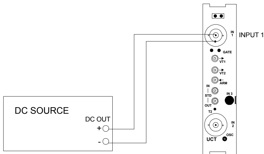
Figure 6-6 Input 1 Trigger Level Test Configuration
