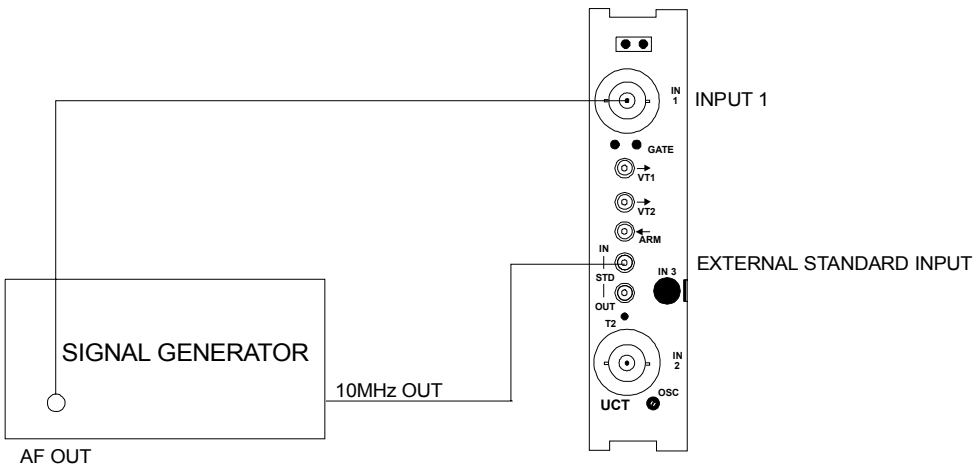
Figure 6-1, Input 1 Low Frequency Sensitivity Test Configuration
