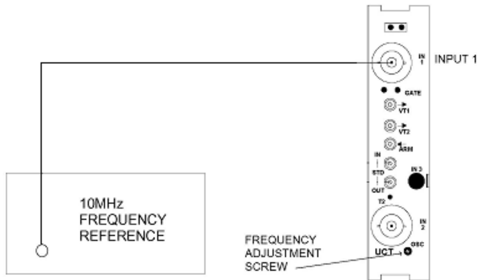
Figure 6-11, External Standard Output
