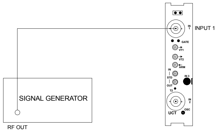
Figure 6-9, Input 1 X10 Attenuator Check Configuration
