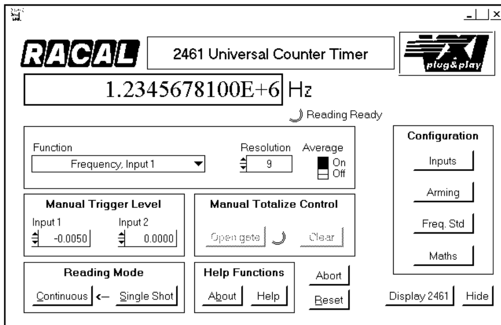
Figure 5-1, 2461-C Front Panel
