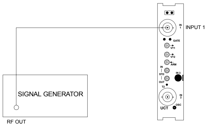
Figure 6-7, Input 1 Filter Check Configuration
