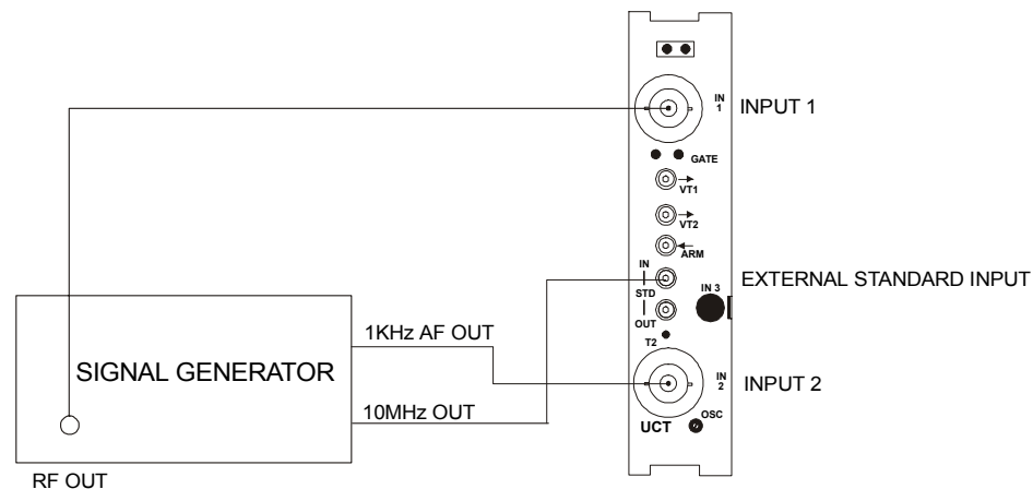
Figure 6-4, Totalize 1 by 2 Test Configuration
