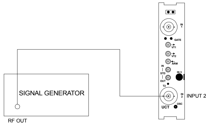
Figure 6-10, Input 2 X10 Attenuator Check Configuration
