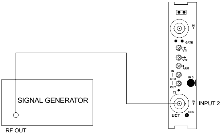
Figure 6-8, Input 2 Filter Check Configuration
