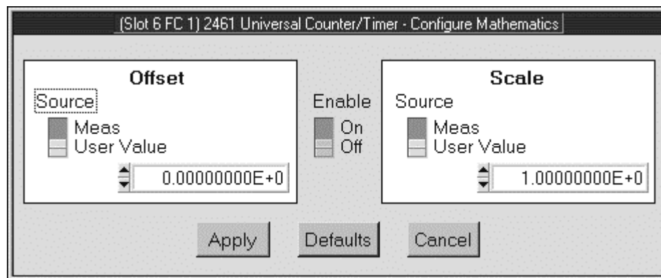
Figure 5-5, Configure Math Function secondary panel
