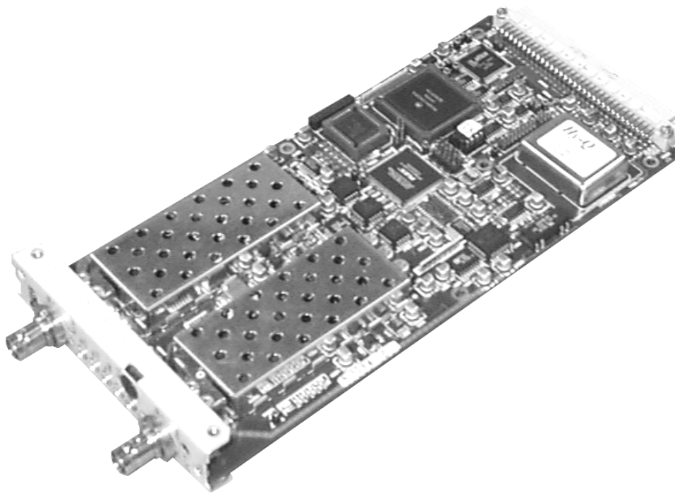
Figure 1-1, Universal Counter Timer 2461 Type C Function Card
