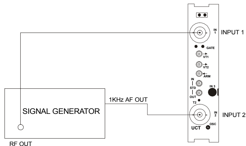
Figure 6-5, Ratio 1 : 2 Test Configuration
