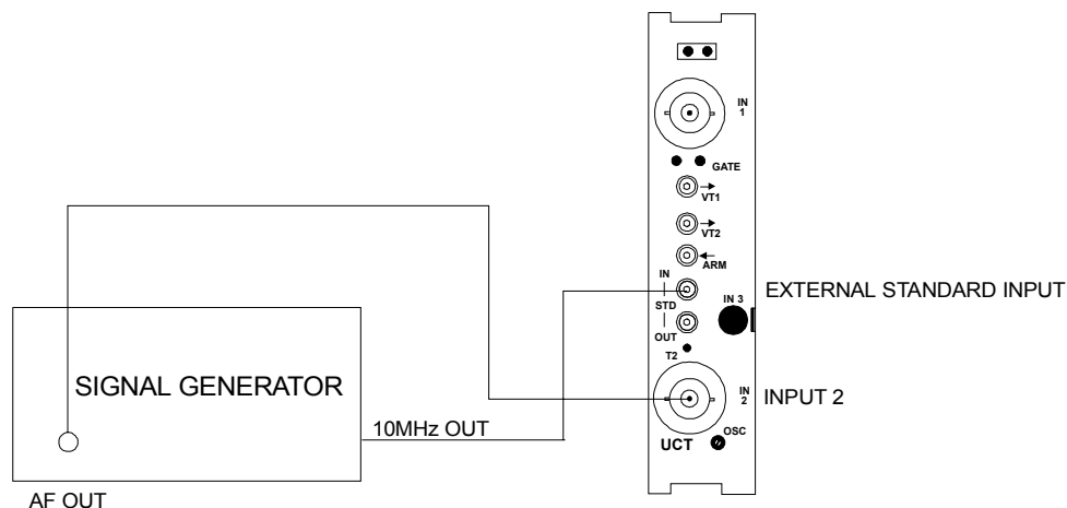
Figure 6-2, Input 2 Low Frequency Sensitivity Test Configuration
