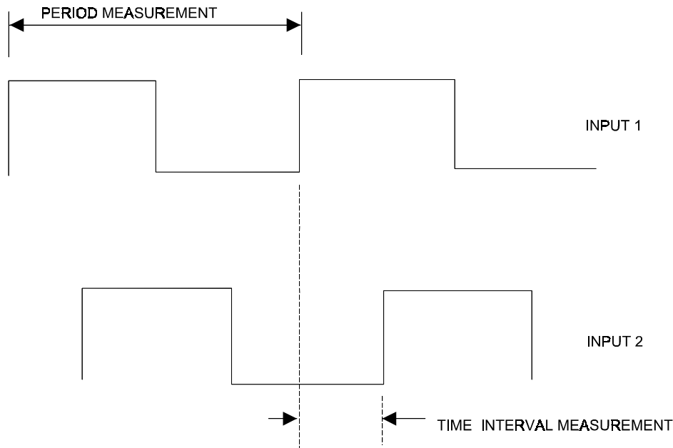
Figure 5-3, Phase Measurement
