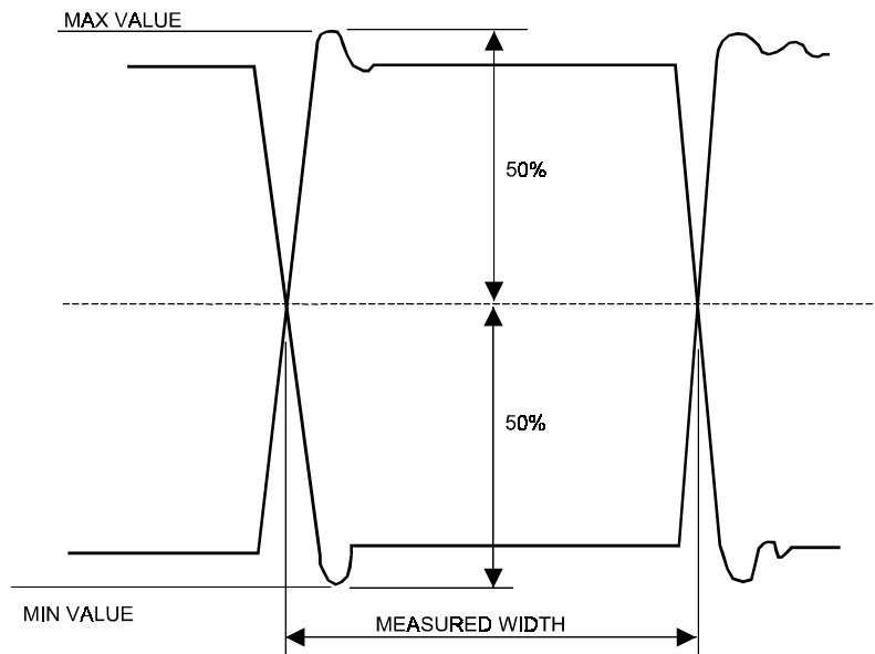
Figure 5-1, Positive/Negative Pulse
