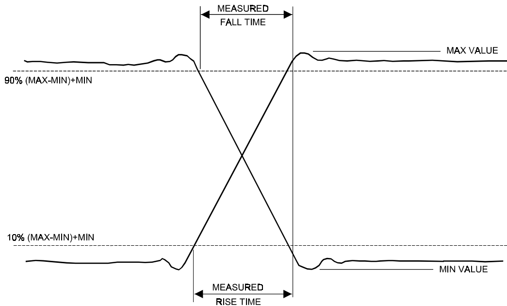
Figure 5-2, Rise/Fall Time
