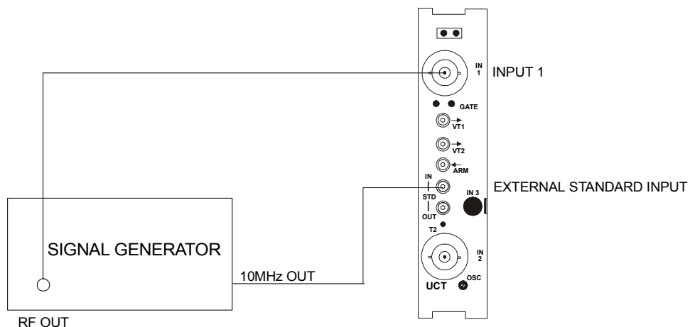
Figure 6-3, Time Interval 1-2 Test Configuration
