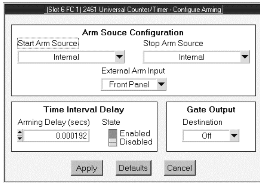
Figure 5-2, Configure Arming secondary panel
