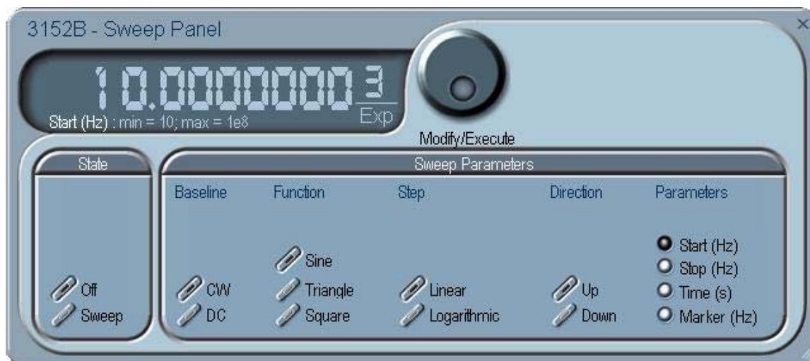
Figure 4-16, Sweep Modulation Panel
