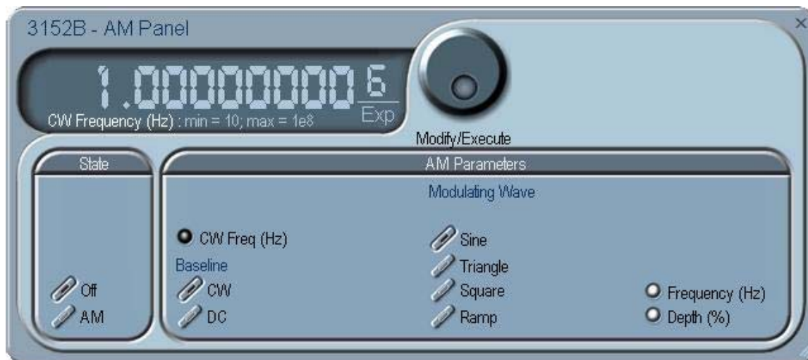
Figure 4-15, AM Panel
