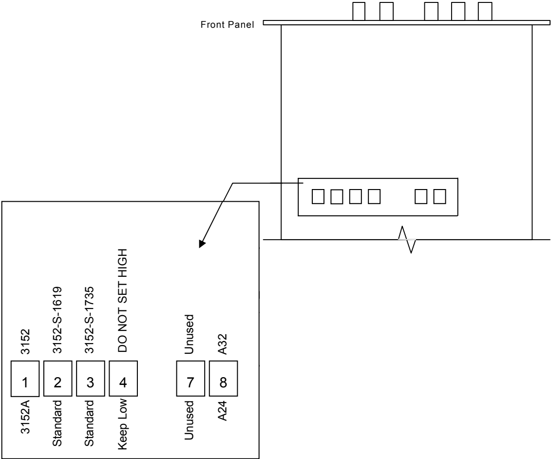
Figure 2-2, 3152 Emulation Mode and Address Space Switch
