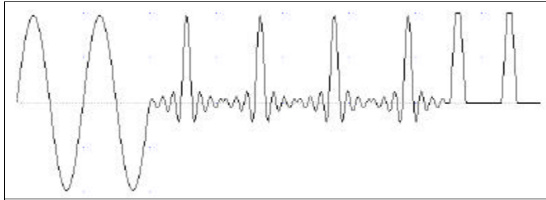
Figure 1-3 Segment 3 - Pulse Waveform
