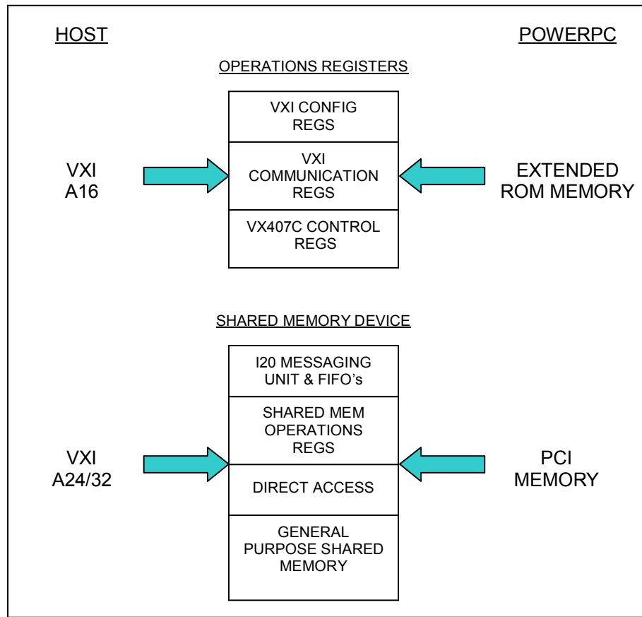
Figure 18 Shared Resources
