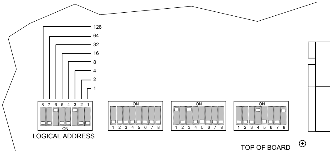
Figure 5 Logical Address Configuration Switch
