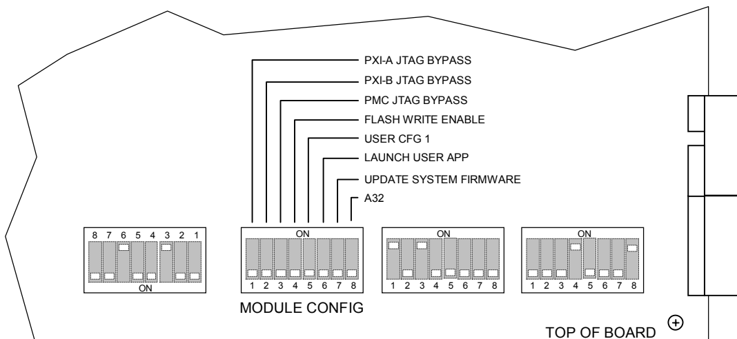
Figure 6 Module Configuration Switch
