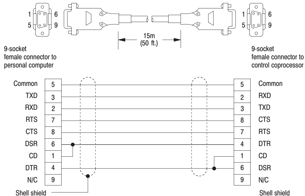
Figure C.1 Cable for a 9-Pin IBM PC/AT, T50, T60, or T47 Computer to the Control Coprocessor 9-Pin COMM0 Port
