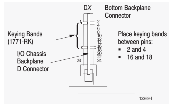
Figure 2.2 Keying Band Positions for the Serial Expander Module
