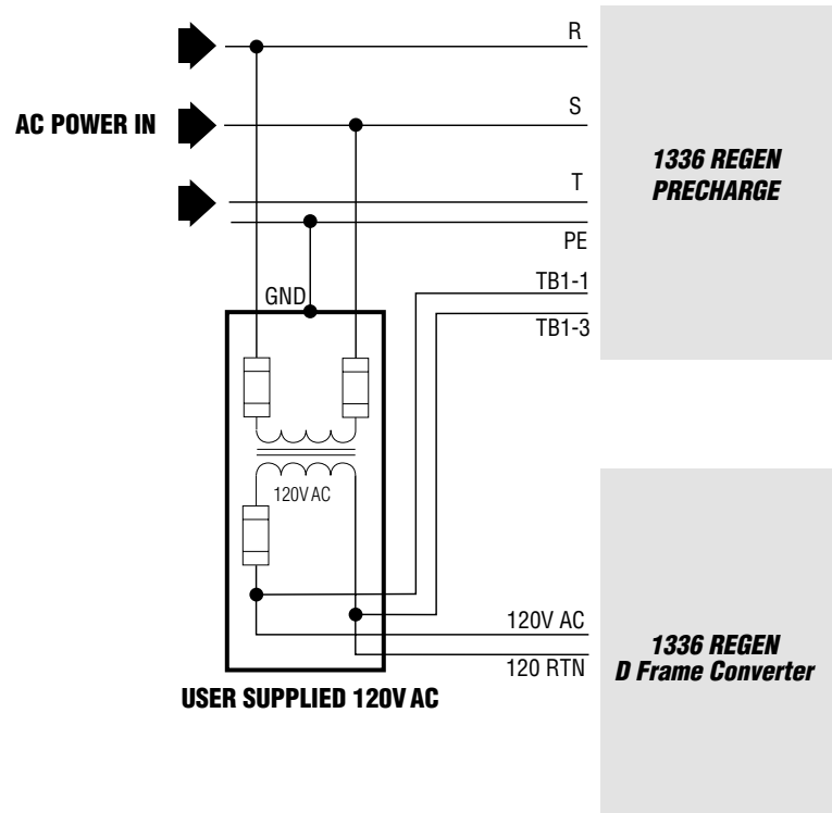
Figure 3.9 — 120VAC Precharge and Converter Connections
