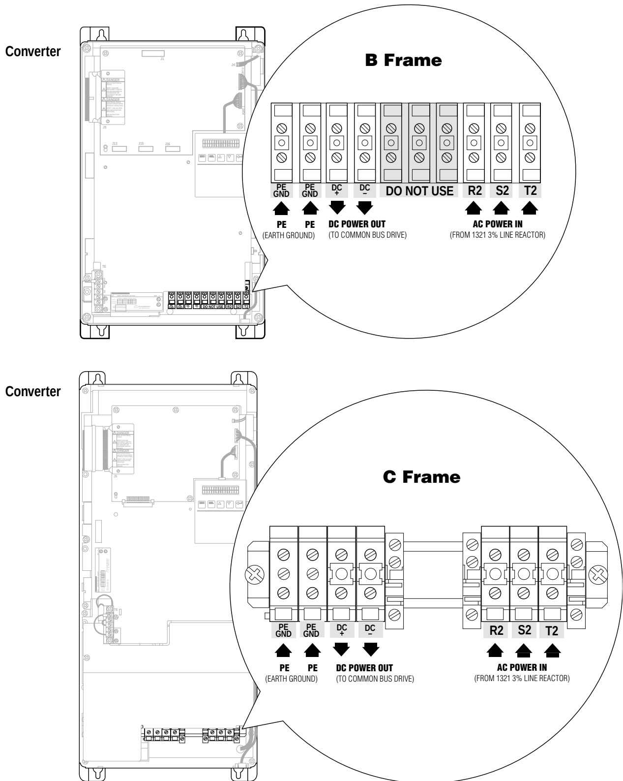
Figure 3.7 — B and C Frame 380-480V AC Converter Connections
