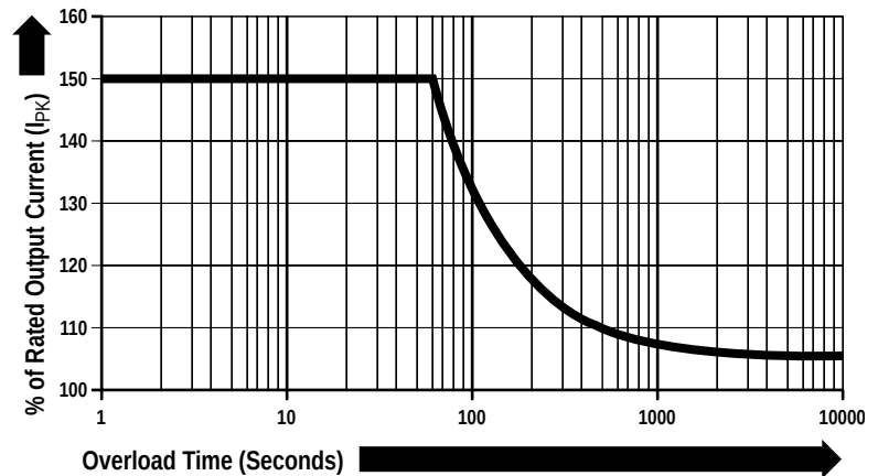
Figure 3.2 — 1336 REGEN Overload Rating
