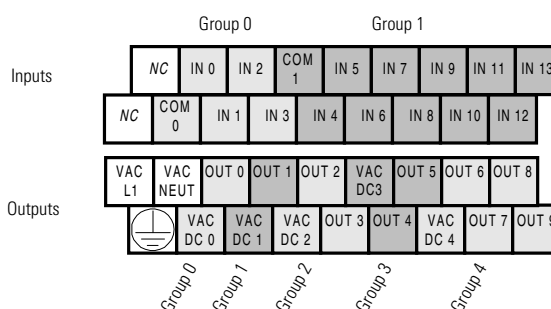
Figure 3.1 1762-L24AWA and 1762-L24AWAR
