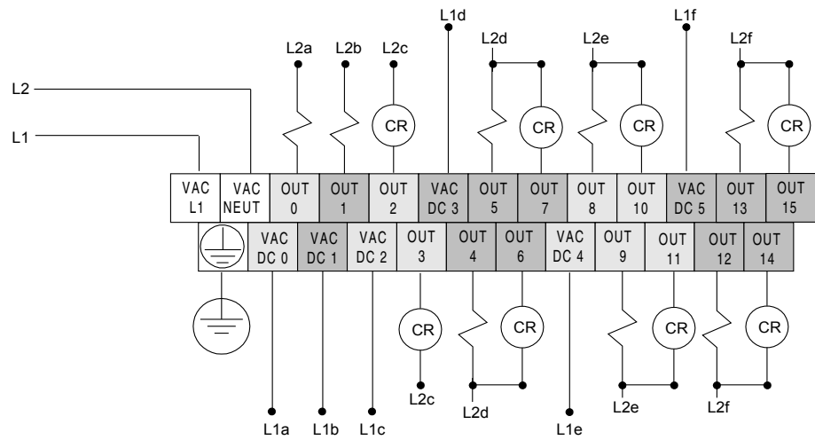
Figure 3.20 1762-L40BXB and 1762-L40BXHR Output Wiring Diagram
