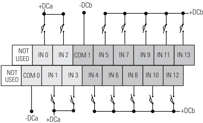
Figure 3.11 1762-L24BXB and 1762-L24BXR Sourcing Input Wiring Diagram
