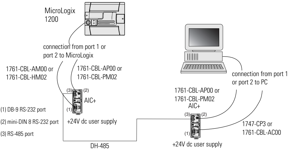
DH-485 Network with a MicroLogix 1200 Controller
