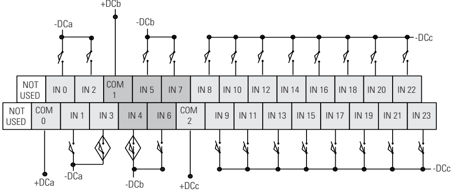
Figure 3.18 1762-L40BXB and 1762-L40BXBR Sourcing Input Wiring Diagram
