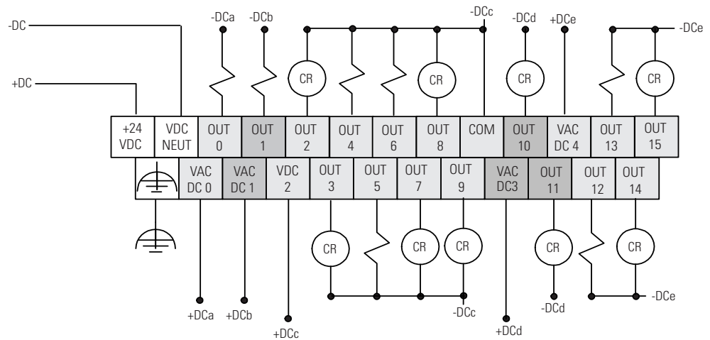
Figure 3.20 1762-L40BXB and 1762-L40BXHR Output Wiring Diagram
