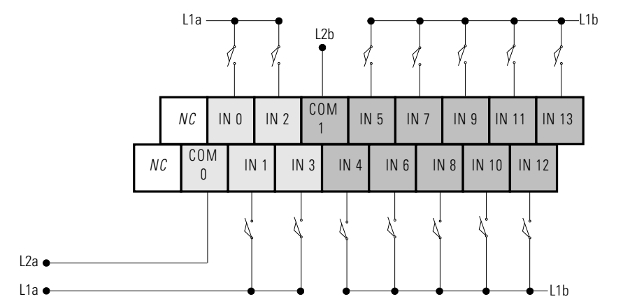
Figure 3.7 1762-L24AWA and 1762-L24AWAR Input Wiring Diagram (1)
