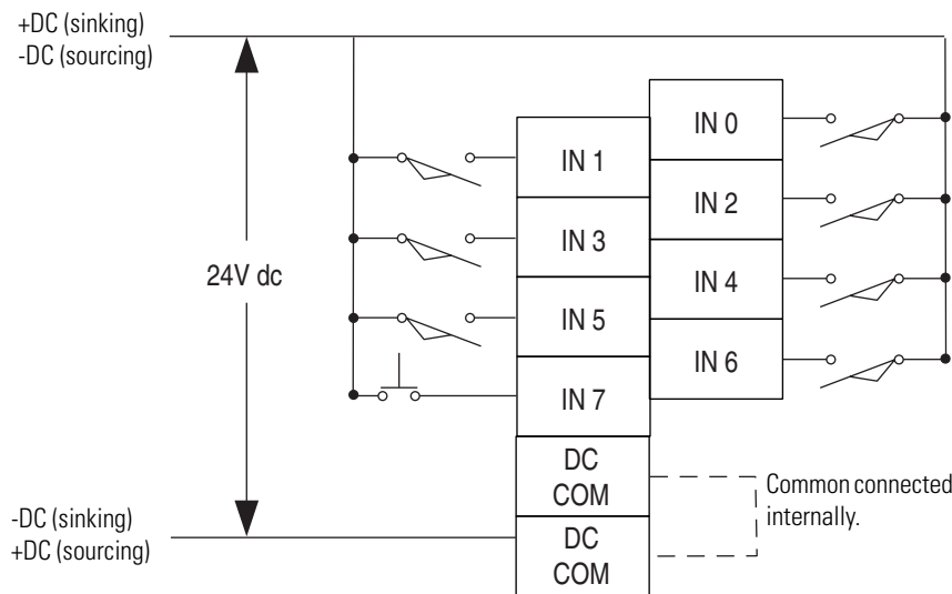
Figure 3.22 1762-IQ8 Wiring Diagram
