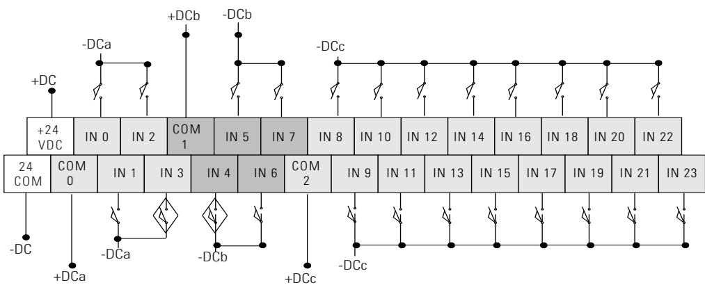
Figure 3.17 1762-L40BXB and 1762-L40BXBR Sinking Input Wiring Diagram
