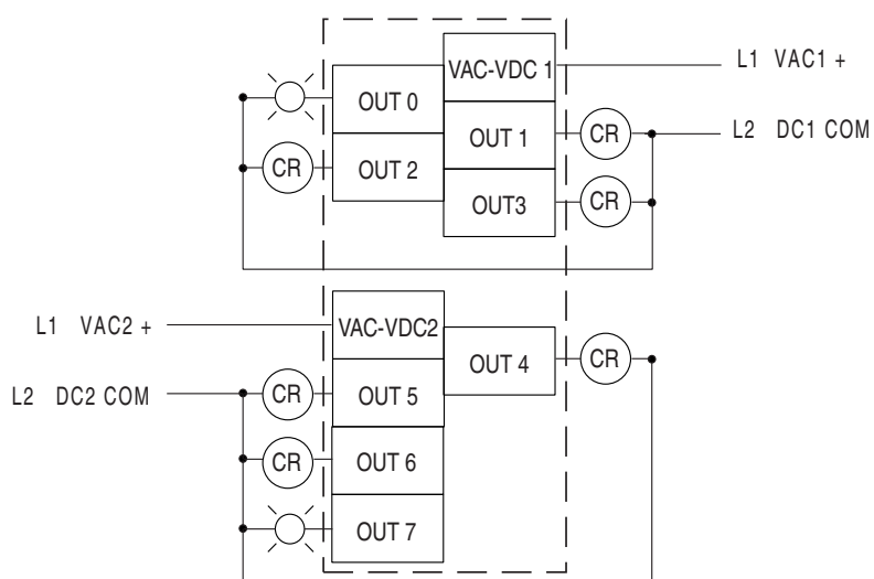
Figure 3.31 1762-OW16 Wiring Diagram
