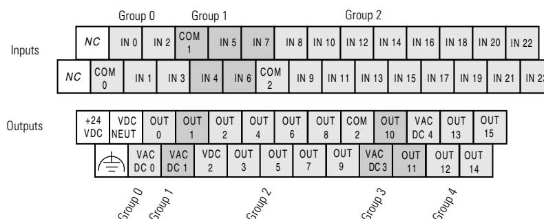
Figure 3.6 1762-L40BXB and 1762-L40BXBR
