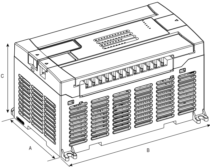
1762-L40AWA, 1762-L40BWA, 1762-L40BXB 1762-L40AWAR, 1762-L40BWAR, 1762-L40BXBR
