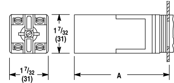
Large Screw Terminals with Pressure Plate Contact Block (Typical View) (1)
