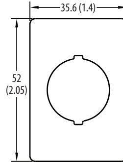
Bulletin 800FC Legend Plate
