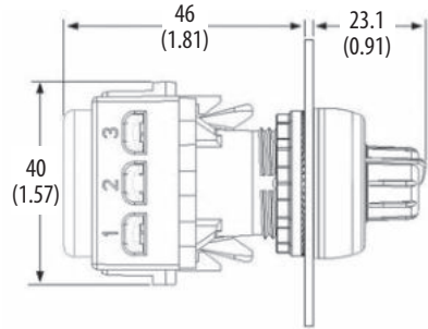
Potentiometer with Resistive Element
