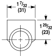
Standard Half Round Legend Plate (1)
