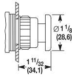
Round Push Button Mushroom
