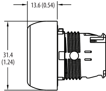
Bulletin 800FC 1-, 2-, and 3-speed Operator
