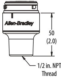
1/2 in. NPT Thread Base
