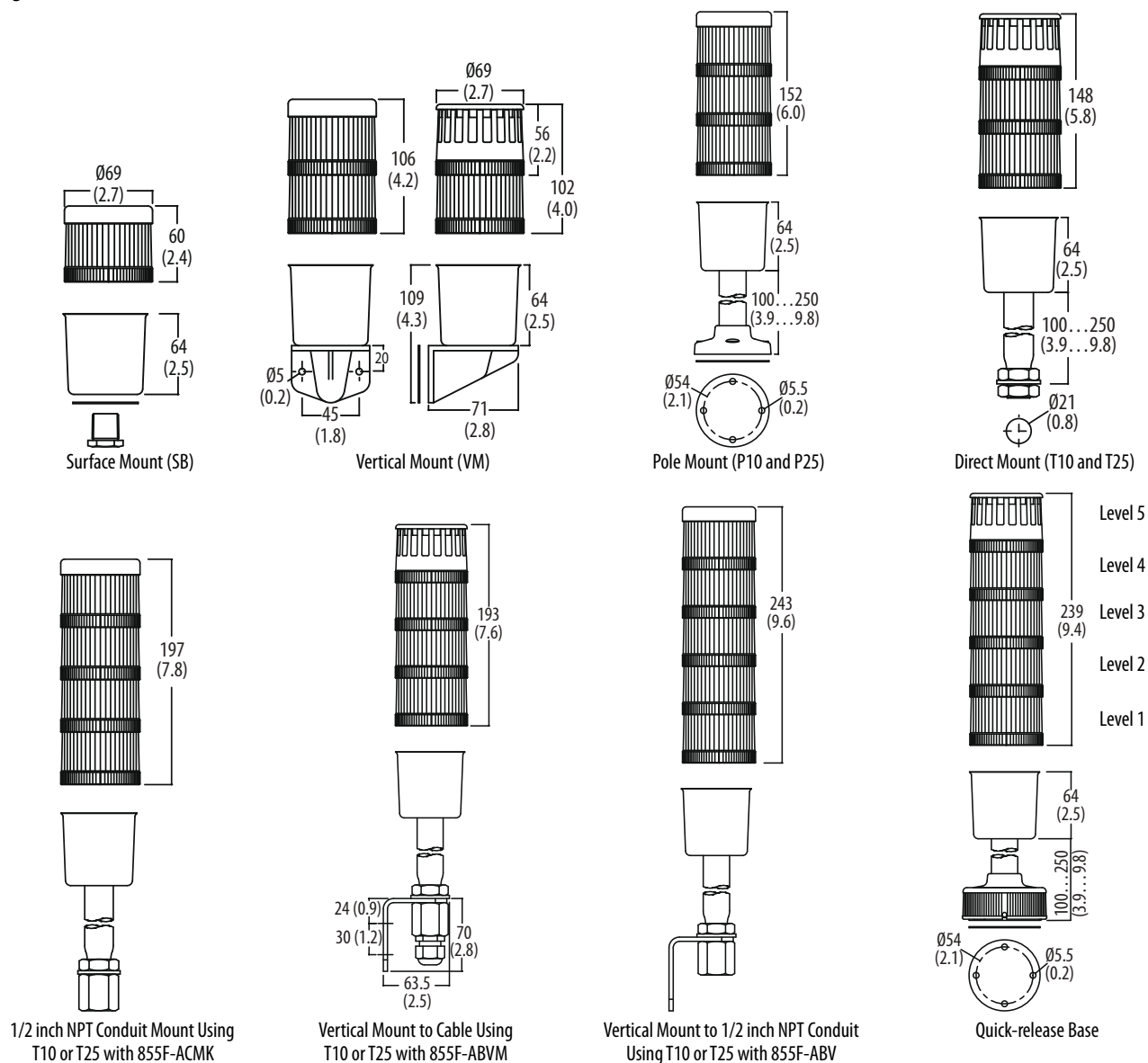
Figure 8 - Assembled Stacks
