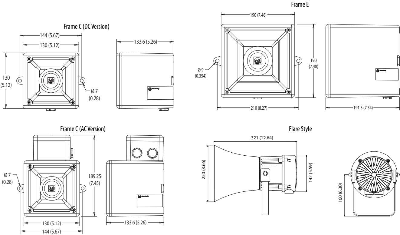
Figure 3 - Recordable Horns
