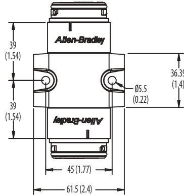
Double-sided Base
