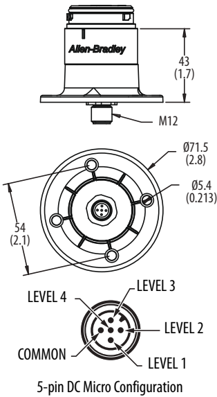
Flange-style Base with M12 Micro Connector (Male)
