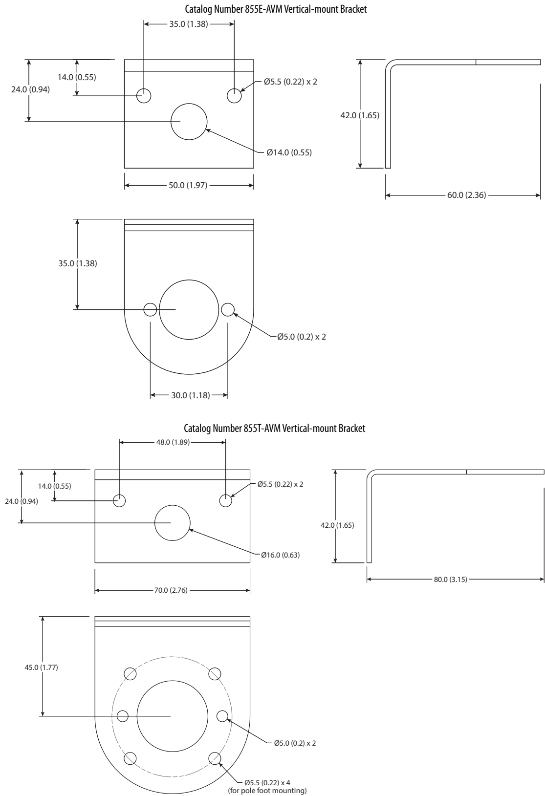
Figure 12 - Component and Accessory Dimensions
