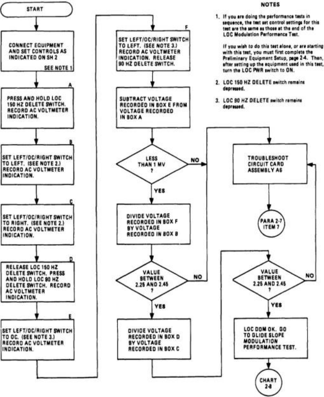
CHART 2-7 LOC DDM Performance Test (Sheet 1 of 2)
