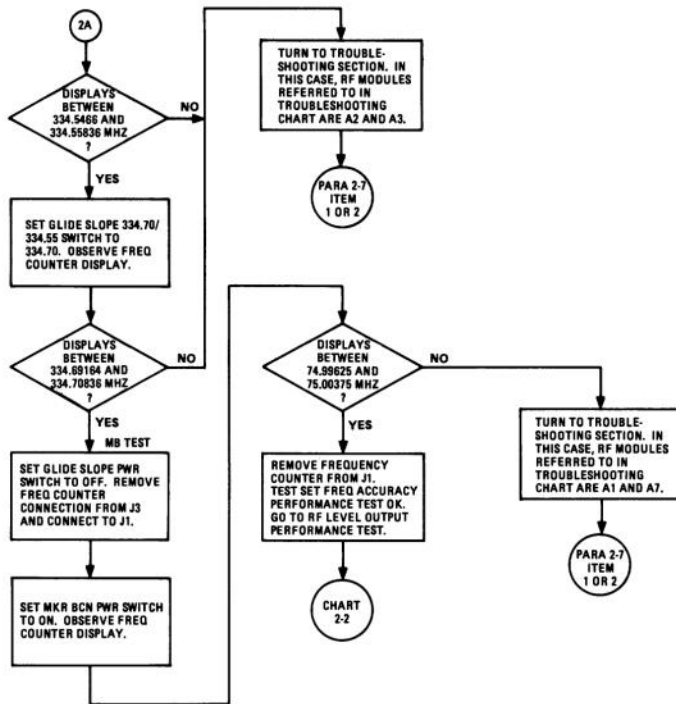
CHART 2-1 Frequency Accuracy Performance Test (Sheet 2 of 3)
