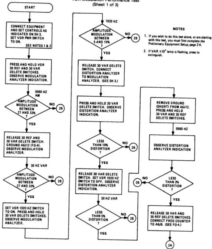
CHART 2-3 VOR Modulation Performance Test (Sheet 1 of 3)
