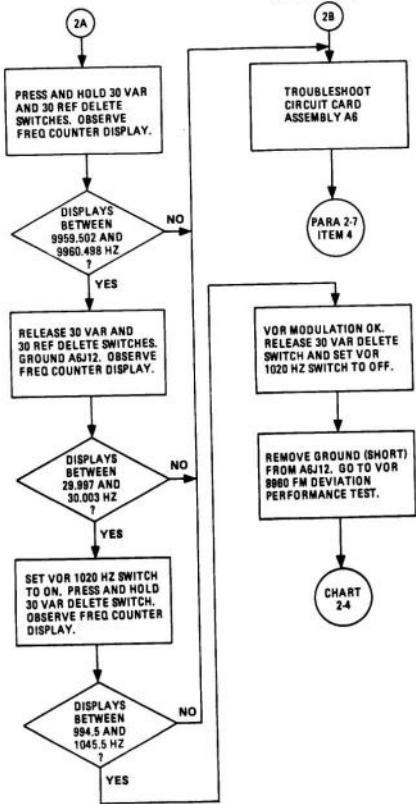
CHART 2-3 VOR Modulation Performance Test (Sheet 2 of 3)
