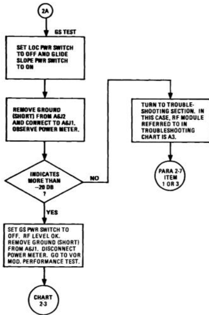
CHART 2-2 RF Level Output Performance Test (Sheet 2 of 3)
