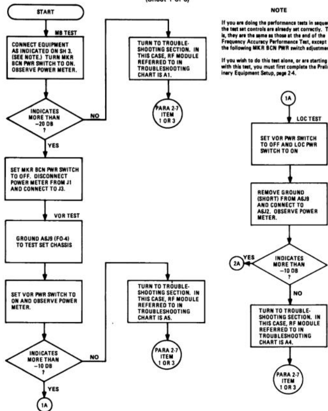
CHART 2-2 RF Level Output Performance Test (Sheet 1 of 3)
