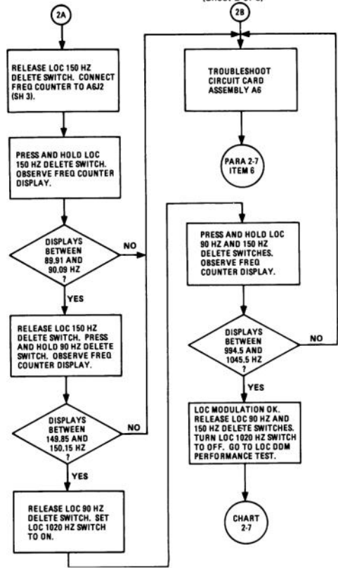
CHART 2-6 LOC Modulation Performance Test (Sheet 2 of 3)
