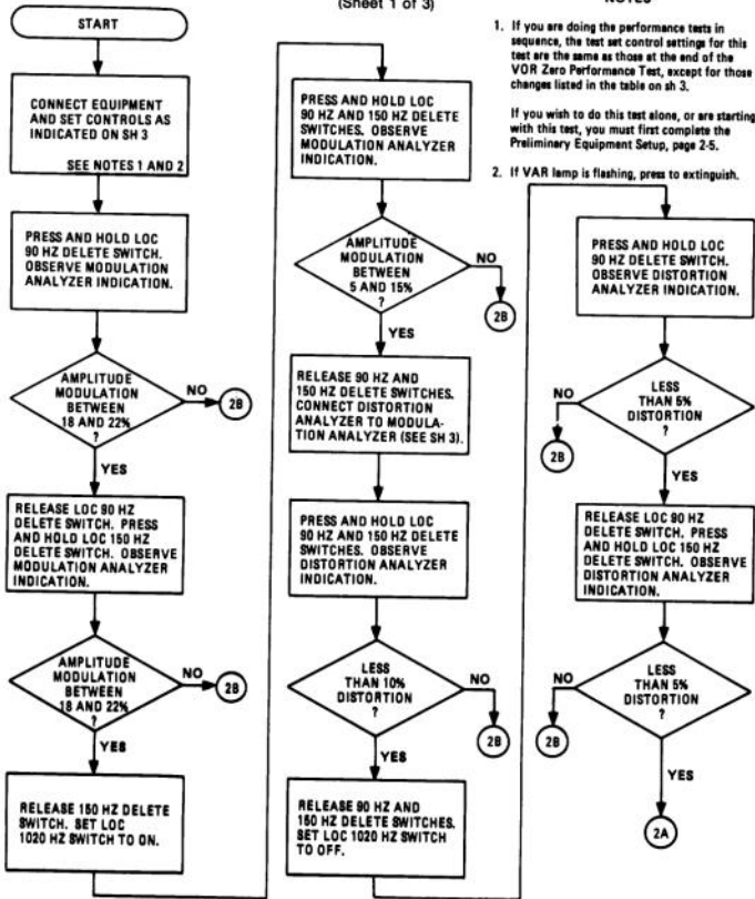
CHART 2-6 LOC Modulation Performance Test (Sheet 1 of 3)
