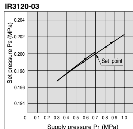
IR3120-03 Back pressure: 1.0 MPa
