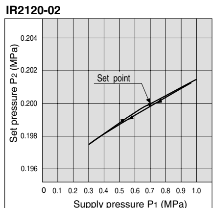
IR2120-02 Back pressure: 1.0 MPa
