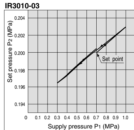
IR3010-03 Back pressure: 0.7 MPa
