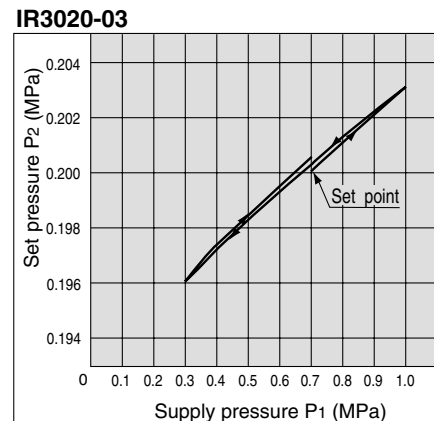
IR3020-03 Back pressure: 1.0 MPa
