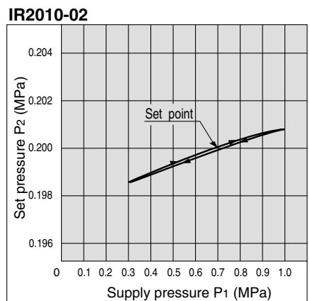
IR2010-02 Back pressure: 0.7 MPa
