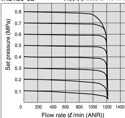
IR2120-02 Supply pressure: 1.0 MPa
