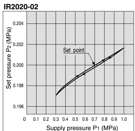
IR2020-02 Back pressure: 1.0 MPa
