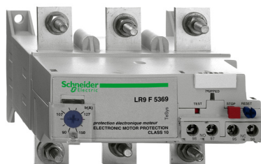
TeSys F Overload Relay LR9F5
