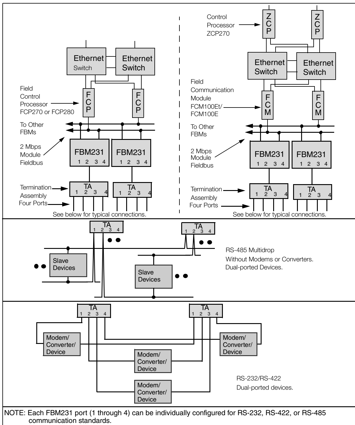
Figure 1. FBM231 in Typical Network Configurations
