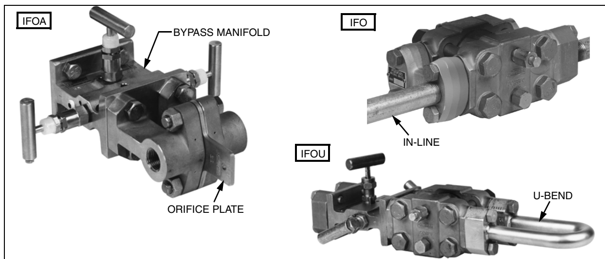
Typical Integral Flow Orifice Configurations
