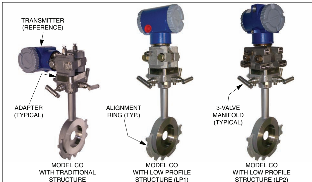
Typical Compact Orifice/Manifold/Transmitter Configurations
