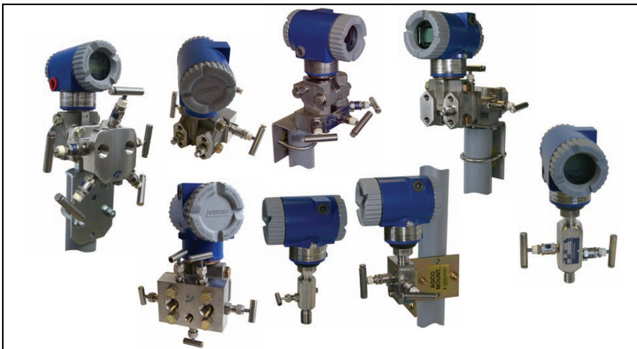
Typical 1-, 2-, 3-, and 5-Valve Manifold/Transmitter Assemblies with AGCO Mounting Bracket, as applicable.
