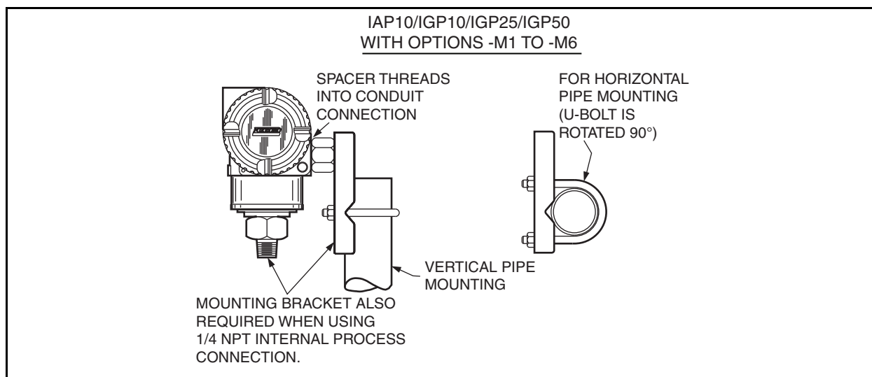
Mounting Bracket Sets for IAP10, IGP10, IGP25, and IGP50 Transmitters
