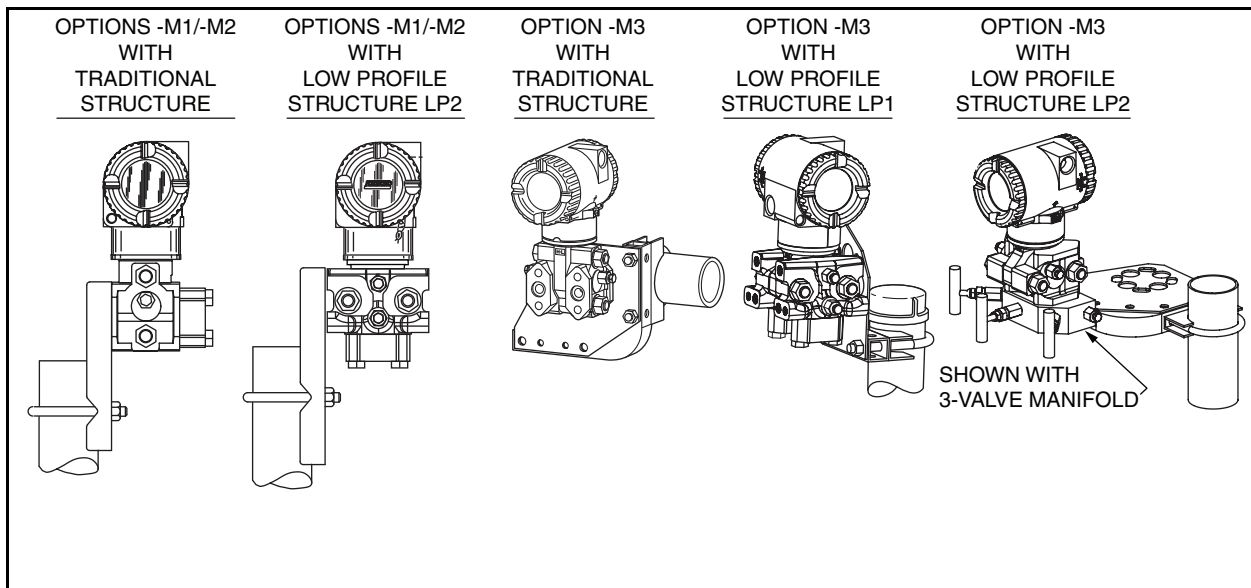
Mounting Bracket Sets for IDP10, IDP25, IDP50, IMV25, IMV30, and IMV31 Transmitters
