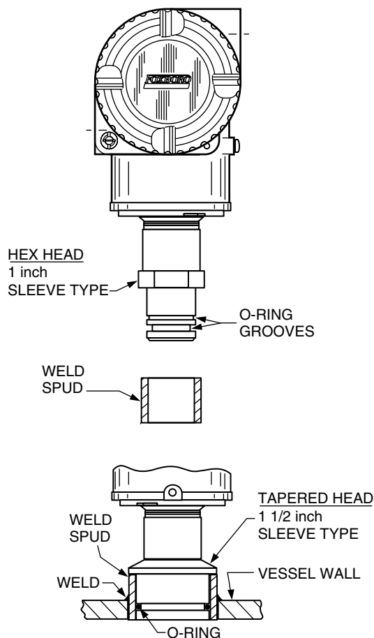
TRANSMITTER WITH INTEGRAL PULP AND PAPER SLEEVE TYPE CONNECTOR
