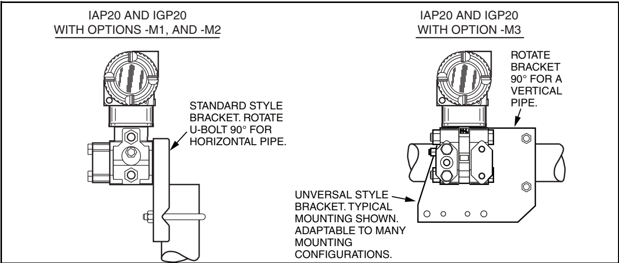
Mounting Bracket Sets for IAP20 and IGP20 Transmitters
