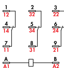
Relay Wiring Diagram Bottom View
