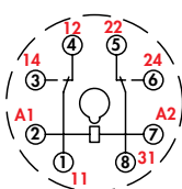
Relay Wiring Diagram Bottom View
