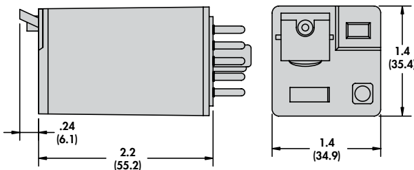
Full Featured Dimensions
