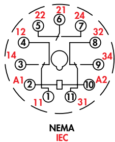
Relay Wiring Diagram Bottom View
