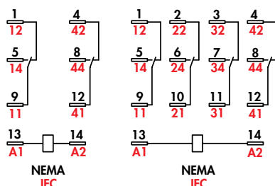
Relay Wiring Diagram Bottom View
