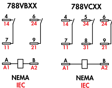
Relay Wiring Diagram Bottom View
