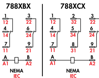
Relay Wiring Diagram Bottom View
