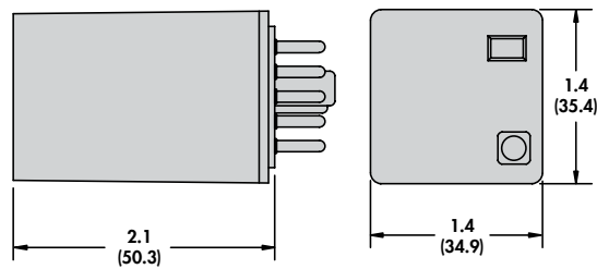
Plain Cover Dimensions
