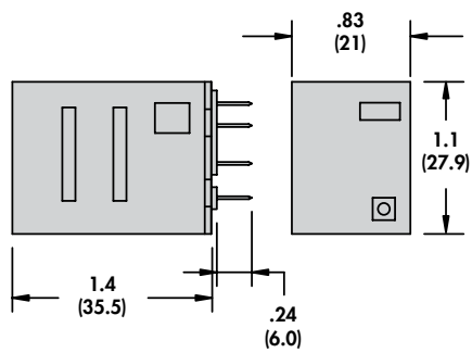
Plain Cover Dimensions
