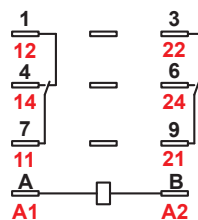
DPDT
