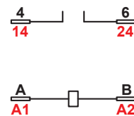
SPST-NO-(DM)
