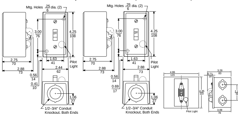
Standard (Class 2510 Types FG & KG, Single Unit)
