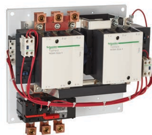
TeSys N reversing starter, Size 4
