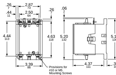
Provisions for #10 or M5 Mounting Screws
