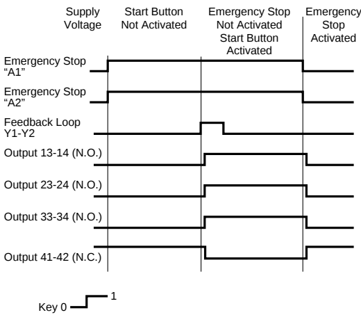
XPSAX Functional Diagram
