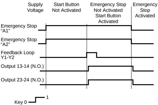
XPSAL Functional Diagram
