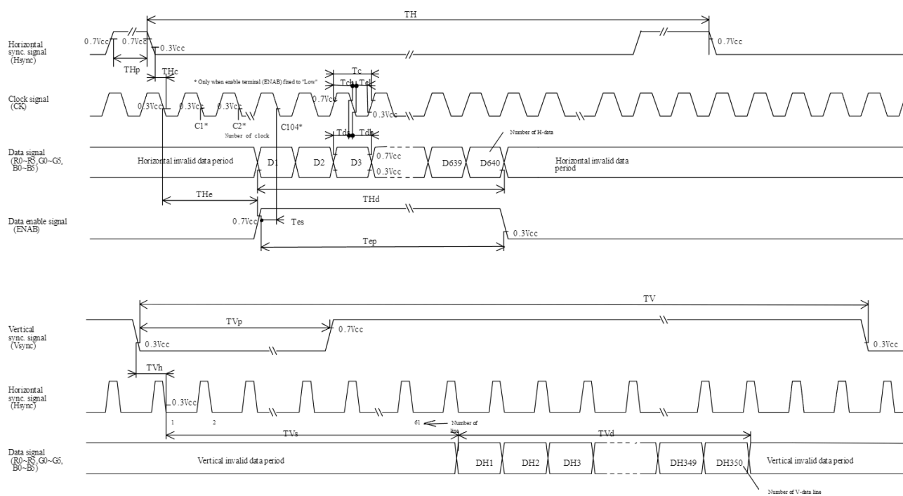
Fig.2-3 Input signal waveforms (350 line mode)
