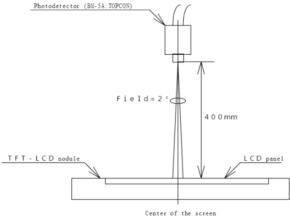
Fig.3 Optical characteristics measurement method
