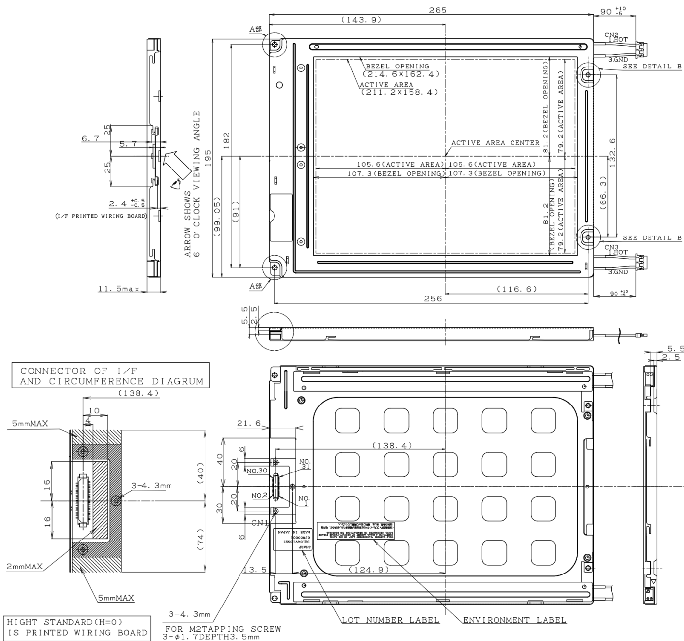
Fig.1 Outline Dimensions
