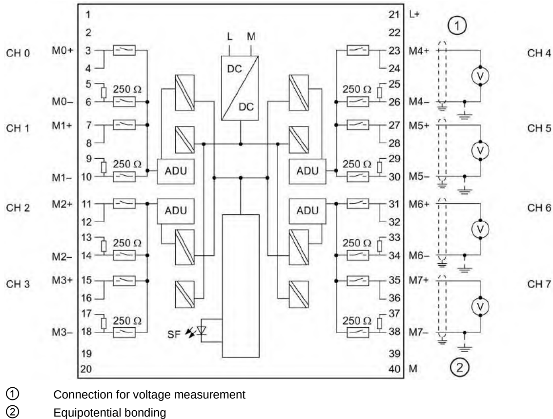
Figure 6-3 Wiring and block diagram
