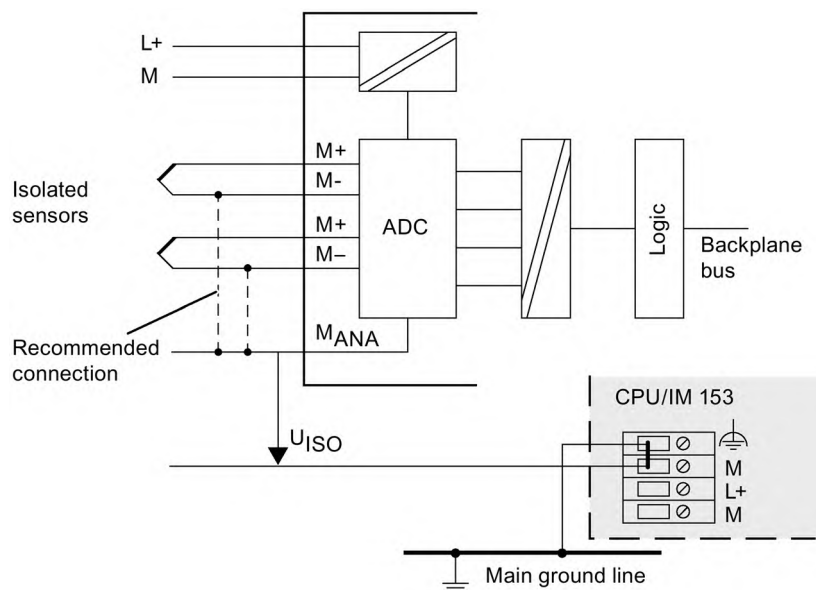
Figure 4-1 Wiring and connecting electrically isolated transducers to electrically isolated AI
