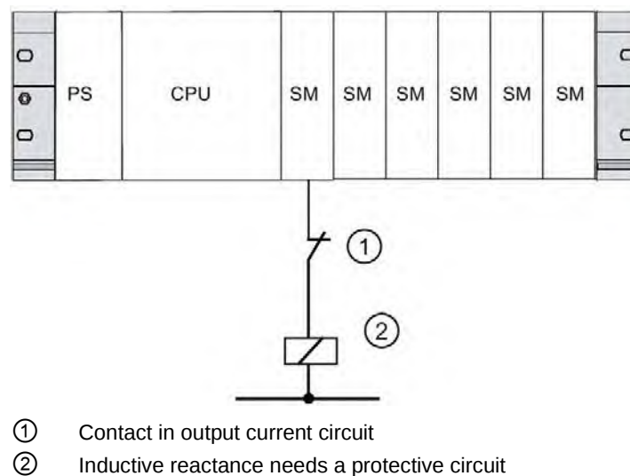
Figure 3-1 Relay contact for emergency stop in output current circuit
