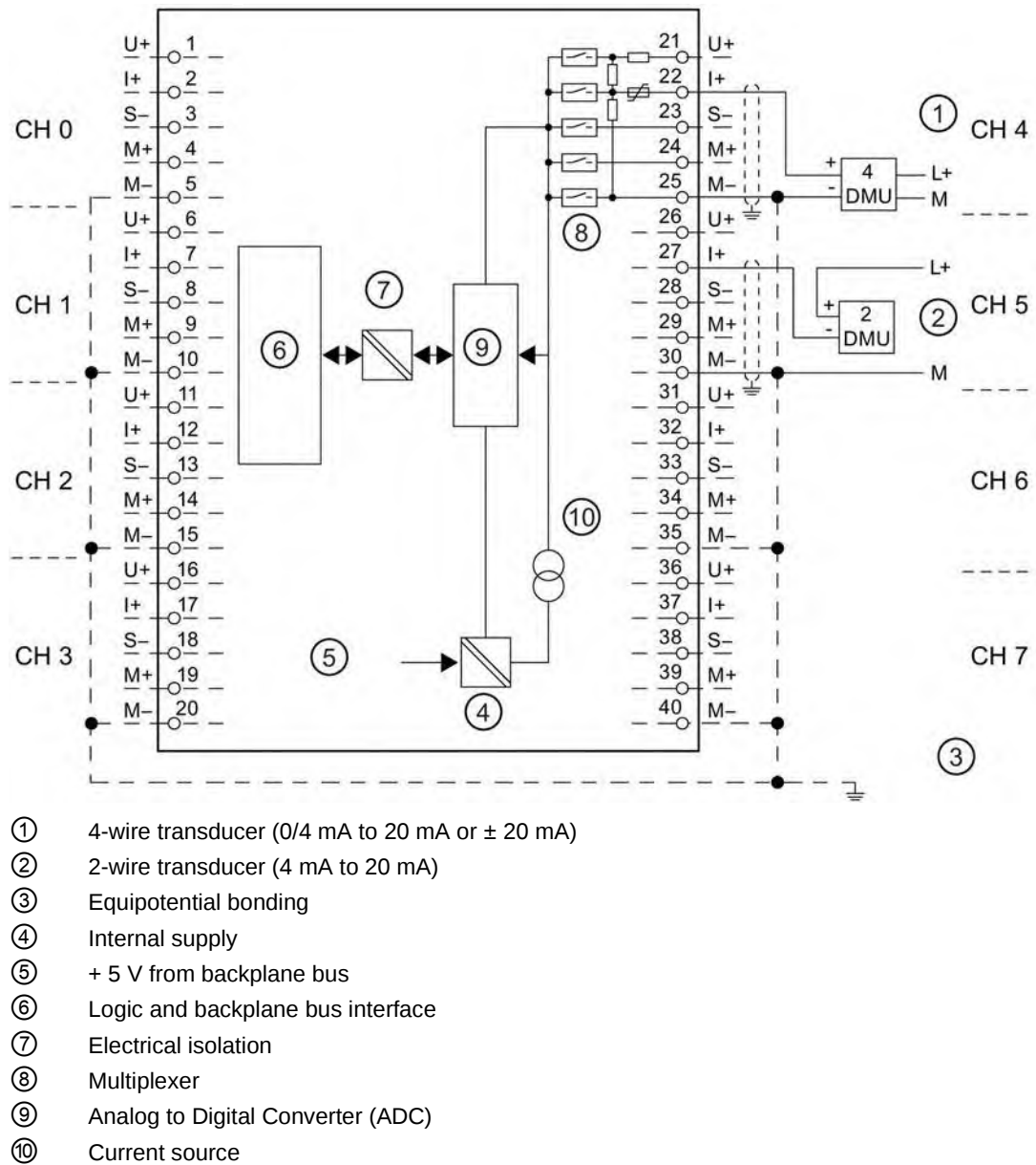
Figure 6-11 Block diagram and wiring diagram
