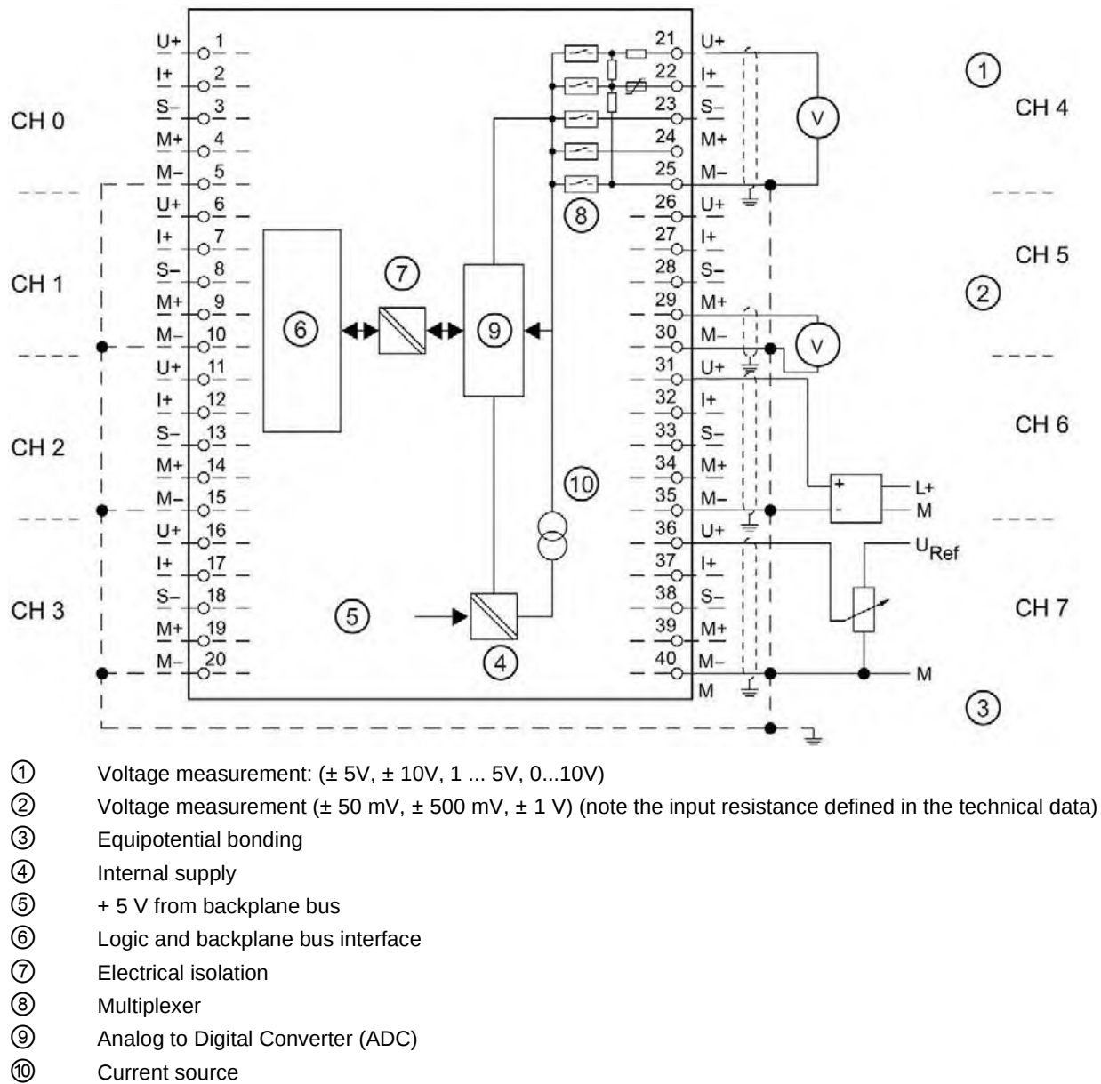
Figure 6-10 Block diagram and terminal diagram
