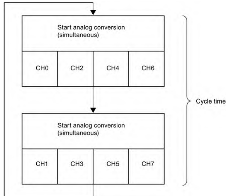
Figure 6-5 8-channel mode cycle time
