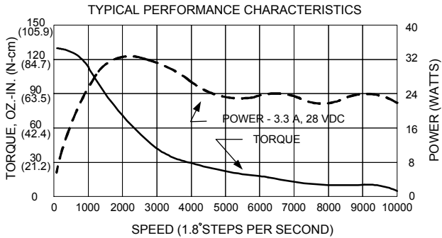
SERIES CONNECTION M062-CS09 AND M062-LS09 MOTORS
