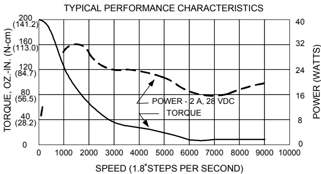
SERIES CONNECTION M063-CS09 AND M063-LS09 MOTORS
