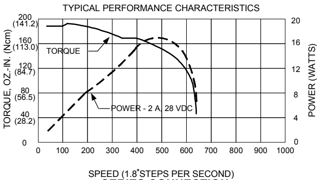
SERIES CONNECTION M063-CS06 AND M063-LS06 MOTORS
