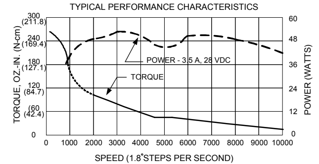
PARALLEL CONNECTION M092-FD8109 AND M092-FD8009 MOTORS
