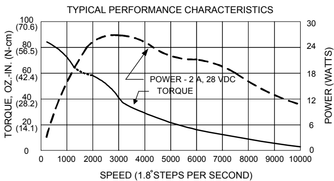
SERIES CONNECTION M062-CS09 AND M062-LS09 MOTORS
