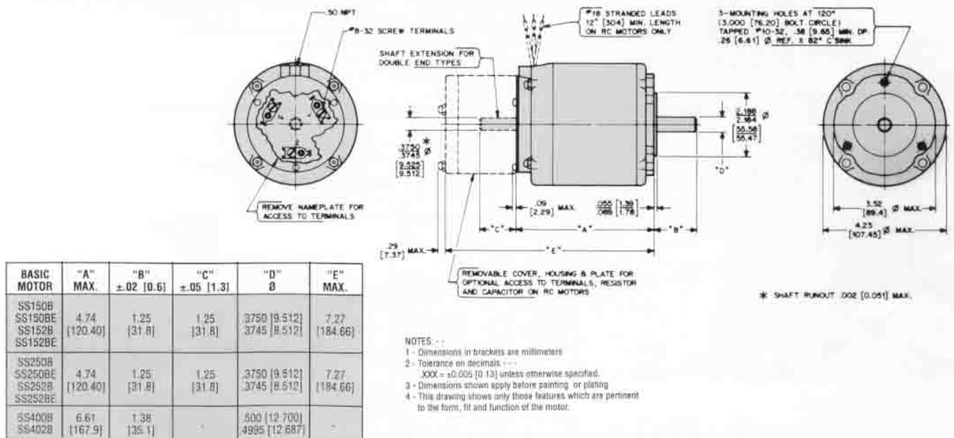
SS150B, SS150BE, SS152B, SS152BE, SS250B, SS250BE, SS252B, SS252BE, SS400B, SS402B Motors
