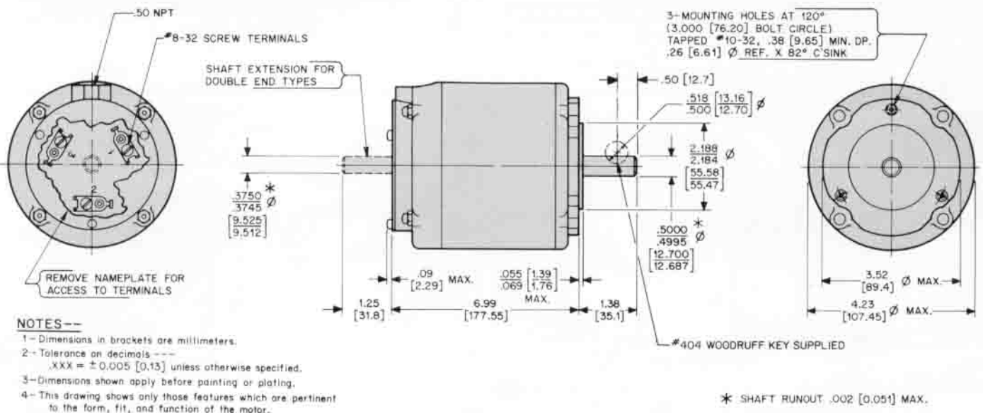
SS700, SS700E, SS702 and SS702E Motors
