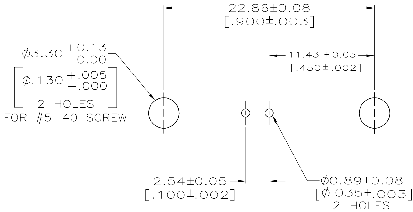
PCB CONFIGURATION
