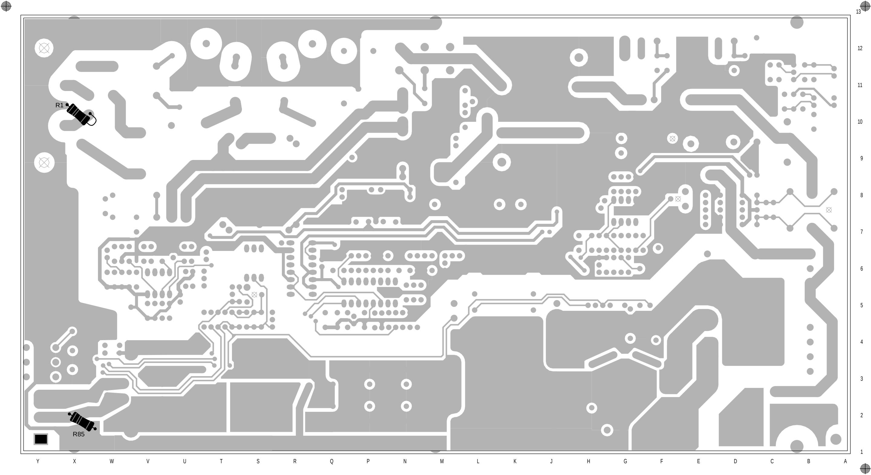
T807/808 PCB Layout Bottom Side 220-01183-03
