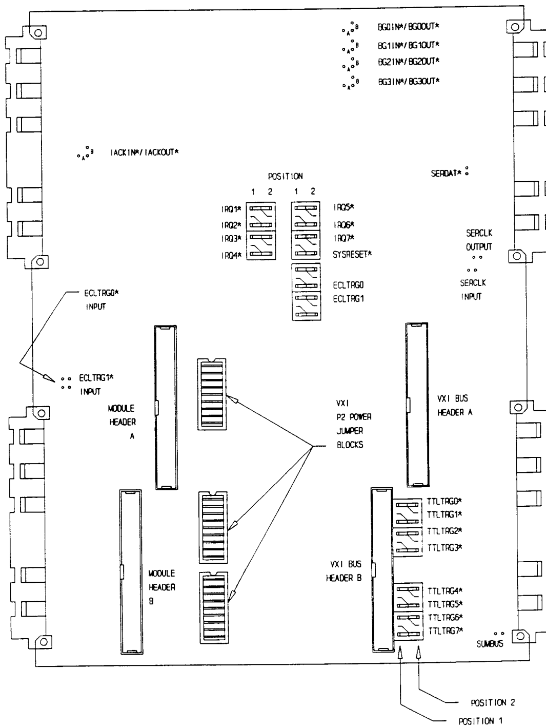
Figure 851-1: 73A-851 Controls and Indicators
