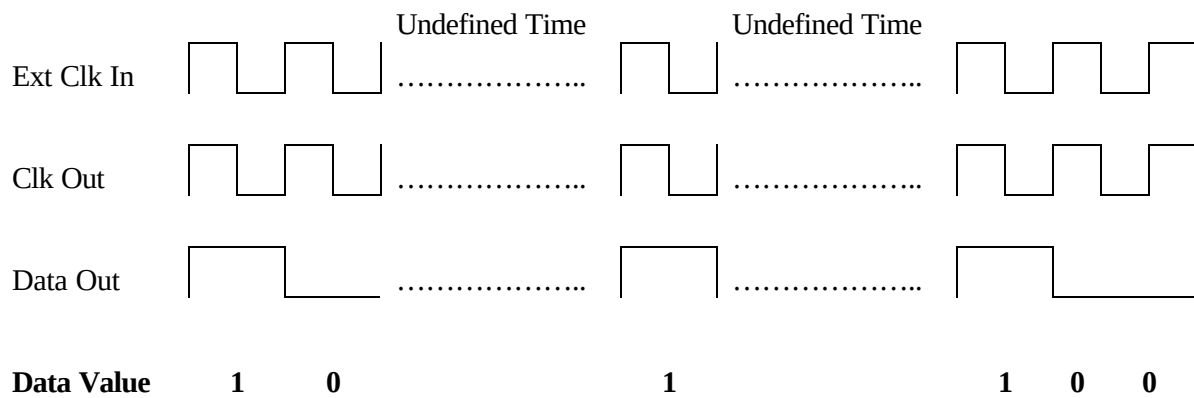
Figure 2-9. Transmitter Burst Mode Option
