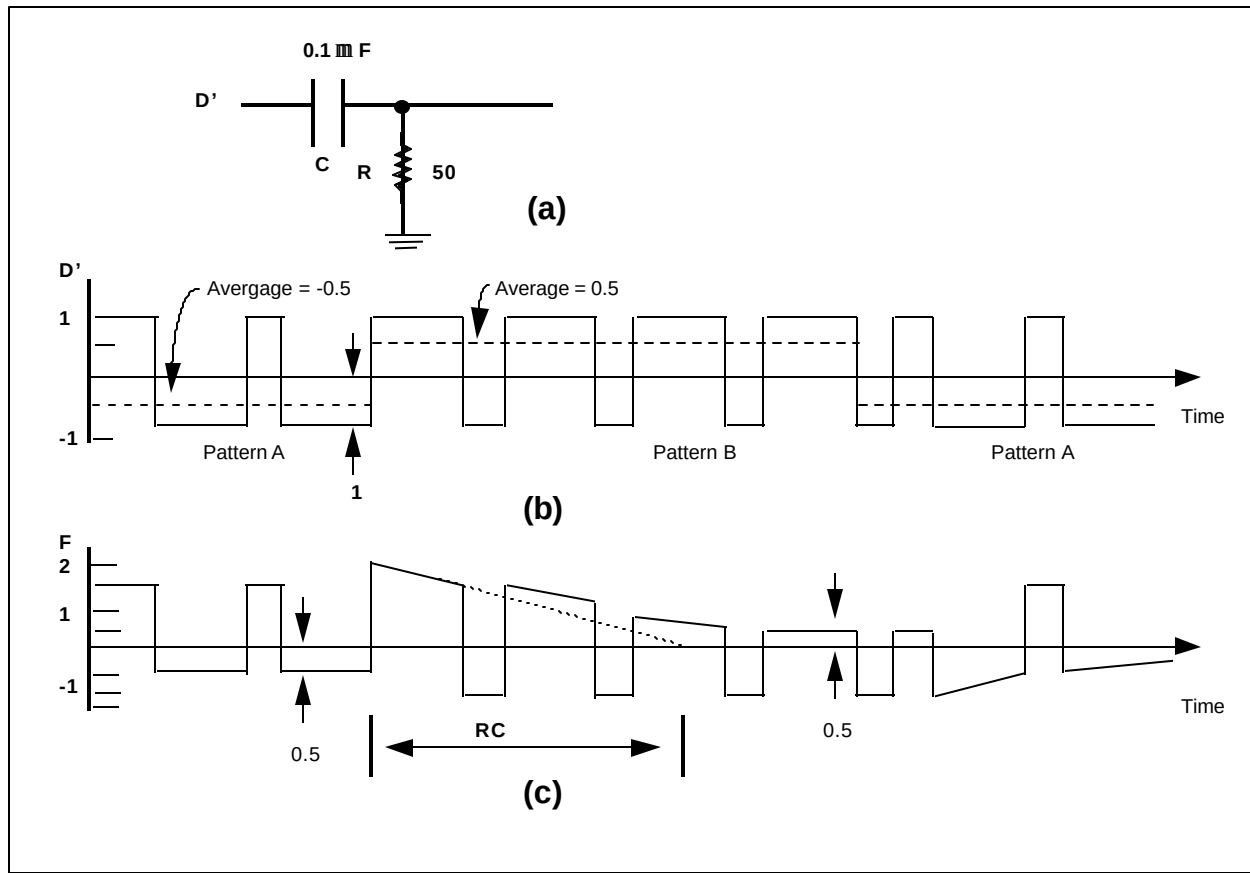
Figure 3. (a) Most transmission systems use AC coupling.
