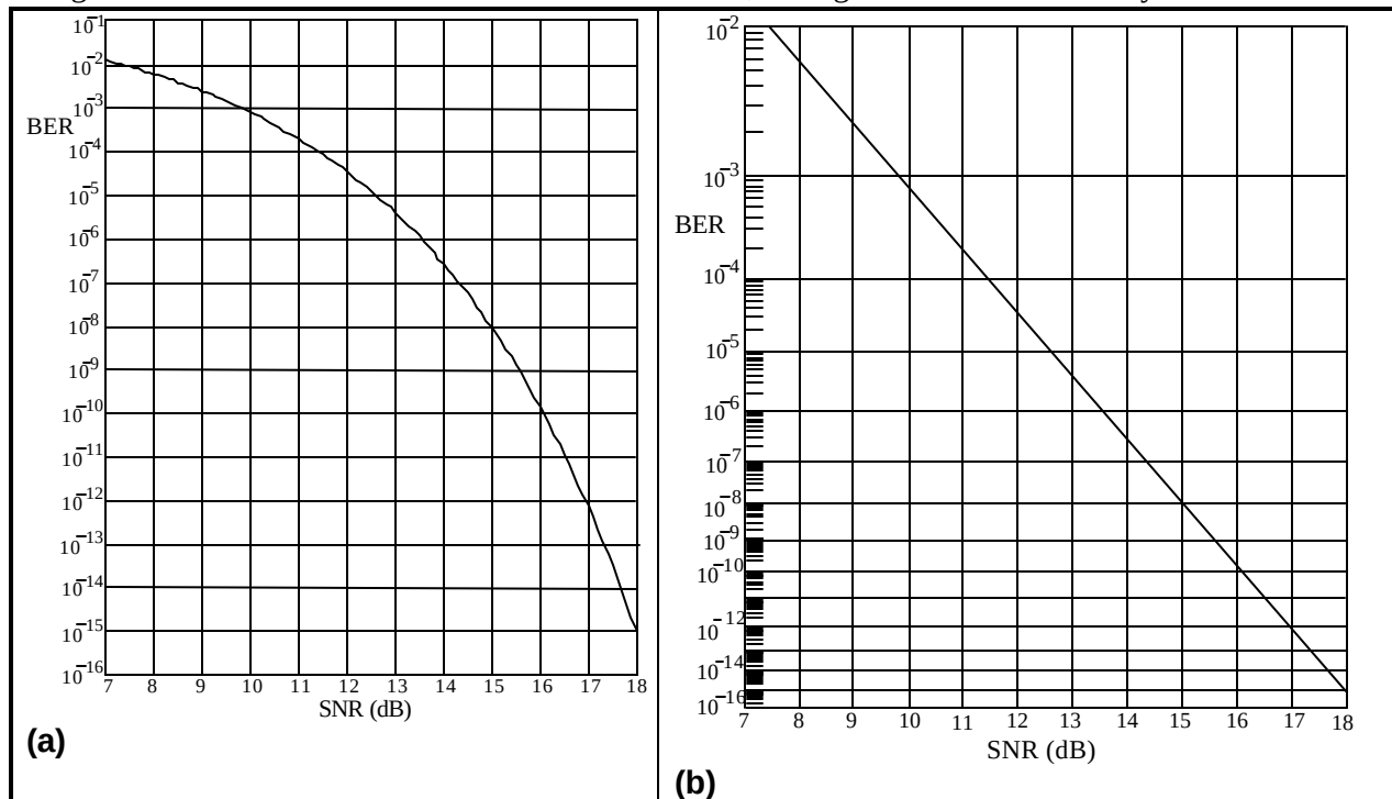
Figure 4. Bit-Error-Rate (BER) is plotted here as a function of the signal-to-noise ratio (SNR), where SNR is S/N_{\text{rms}} in decibels (electrical), S is the distance from the signal (1 or 0) to the decision threshold and N_{\text{rms}} is the rms value of the Gaussian noise introduced by the first receiver state (a). In (b), the log scale was distorted, so the plot is a straight line.
