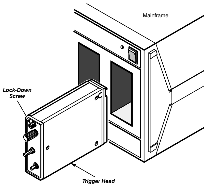
Figure 3: Installing a Trigger Head in an Instrument
