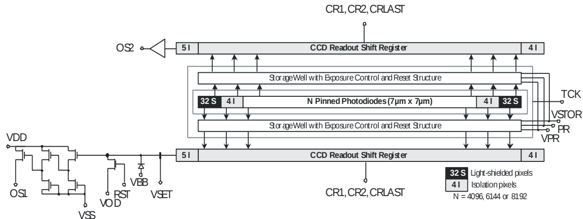
Figure 3: IL-P4 Image Sensor (4k (7 \mu m), 6k, and 8k, 2 tap models)
