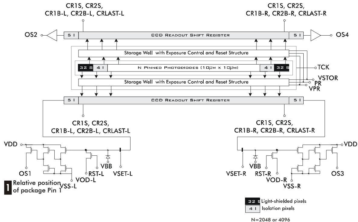
Figure 2: IT-P1 4k Image Sensor (2k, 4k (10 \mu\text{m} ), 4 tap models)
