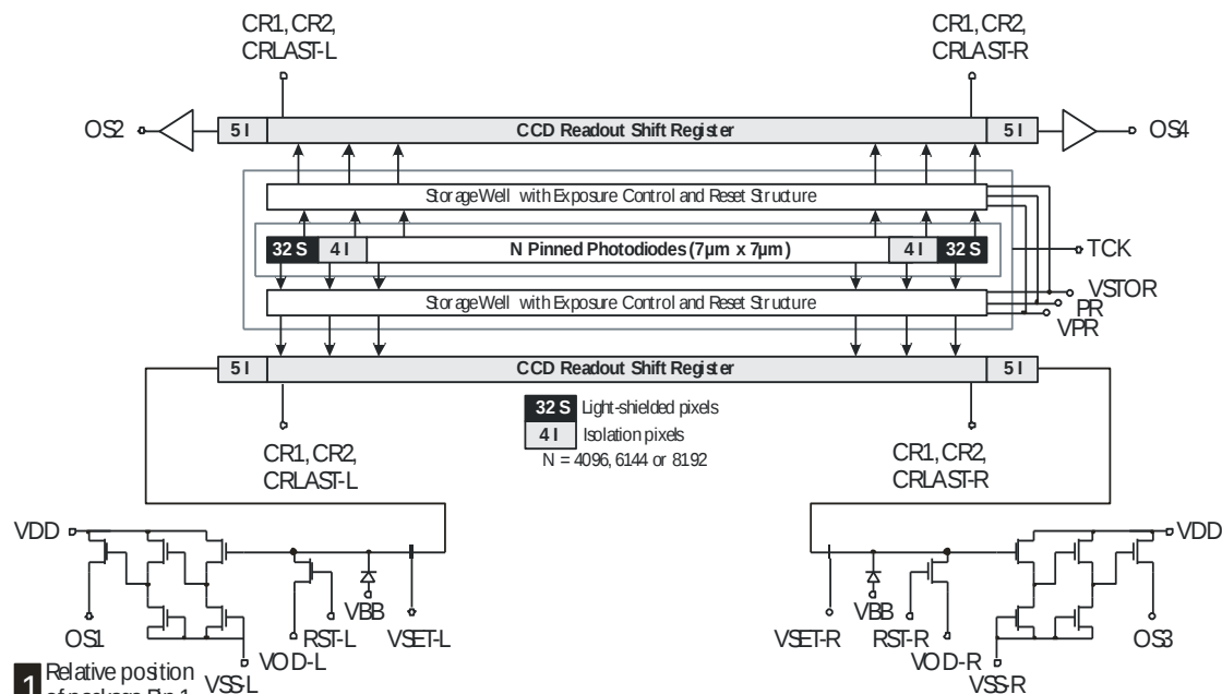
Figure 4: IT-P4 Image Sensor (4k (7 \mu m), 6k, and 8k, 4 tap models)
