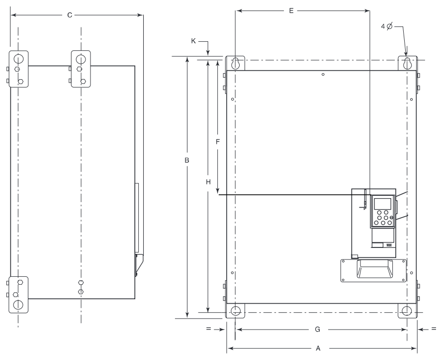
Figure 4: Frame Size 9
