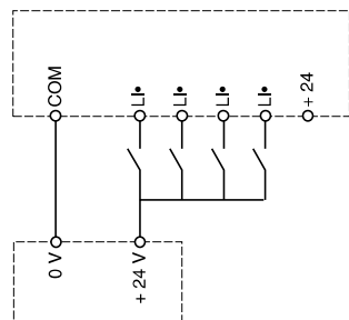
Figure 27: External Supply Wiring Diagram
