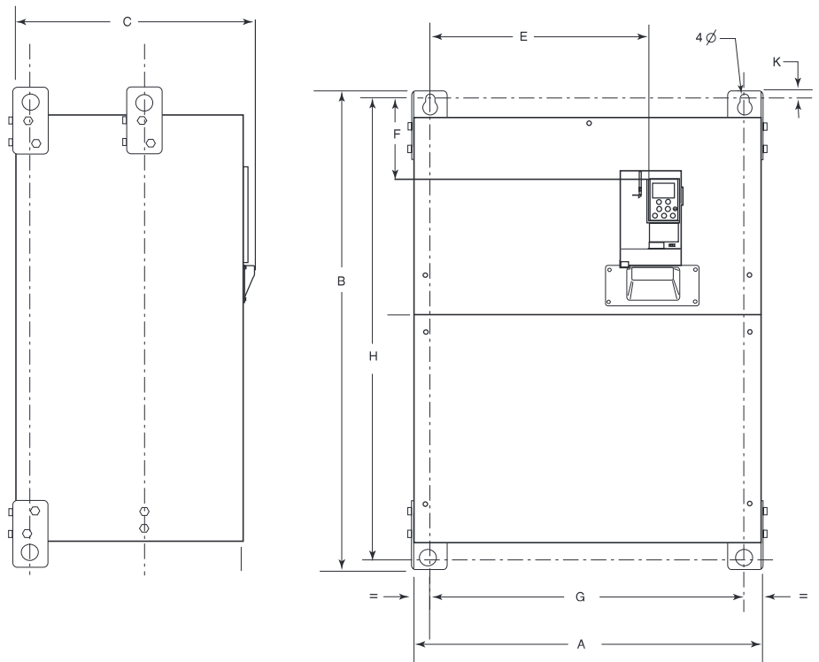
Figure 5: Frame Size 10
