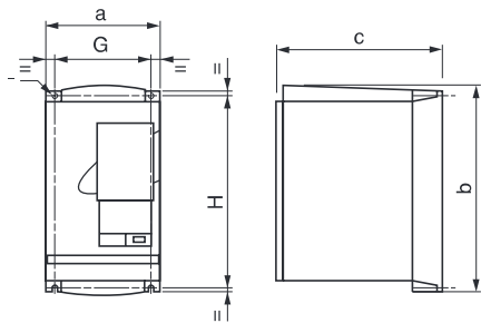
Figure 1: Frame Sizes 1–5
