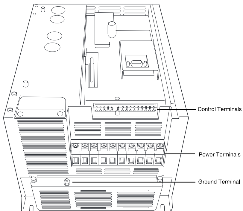
Figure 13: Terminal Locations (Frame Sizes 4 and 5)
