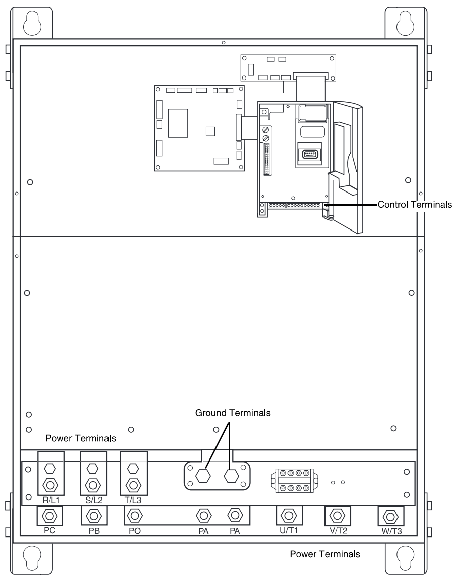
Figure 18: Terminal Locations (Frame Size 10)
