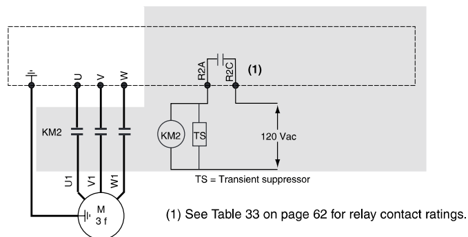
Figure 26: Output Contactor Wiring Diagram
