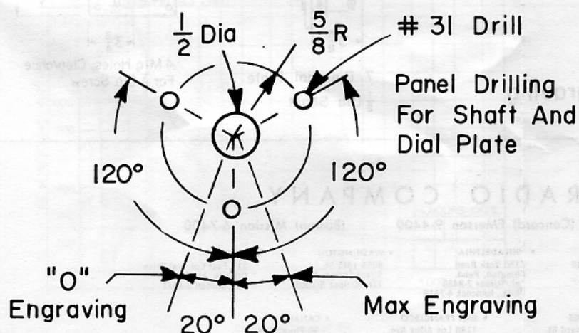
Figure 7. Mounting Dimensions
