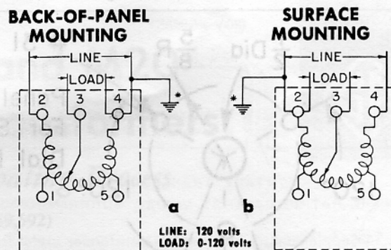
Figure 6. Recommended line-voltage connections
