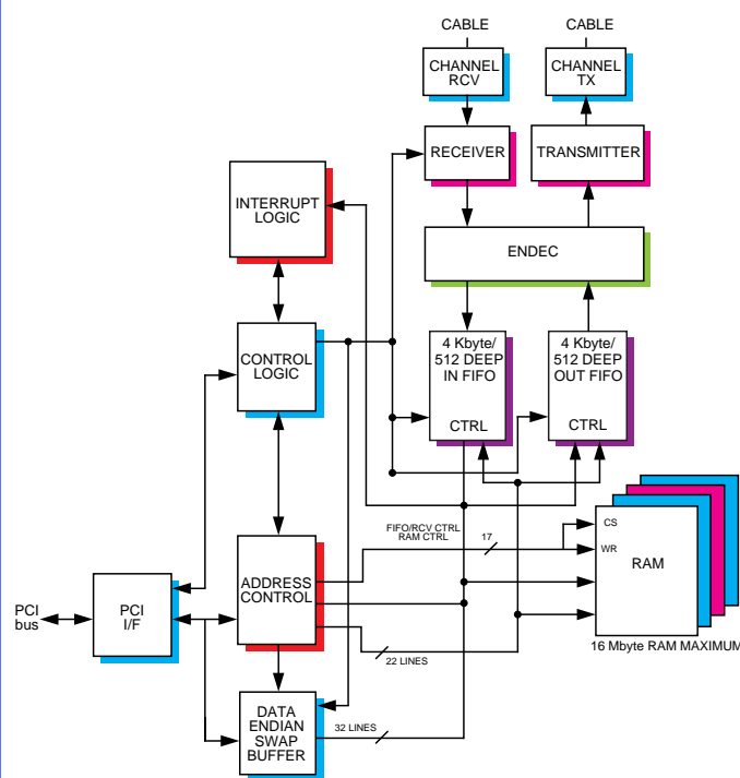
Figure 2. VMIPCI-5588 Functional Block Diagram
