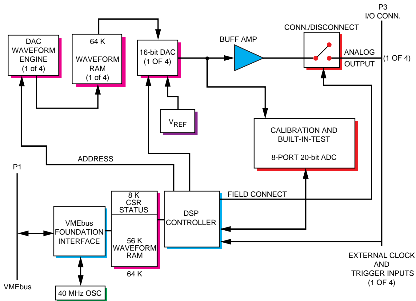
Figure 1. VMIVME-4145 4-Channel Arbitrary Waveform Analog Generator Board with Autocalibration Functional Block Diagram
