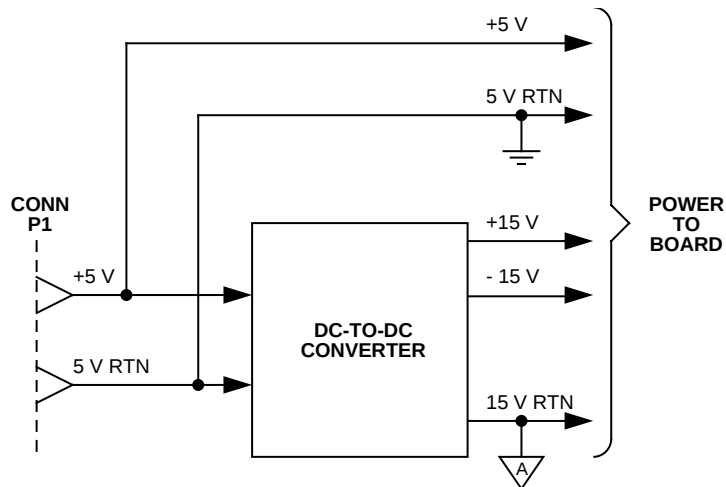
Figure 1-6 Power Converter
