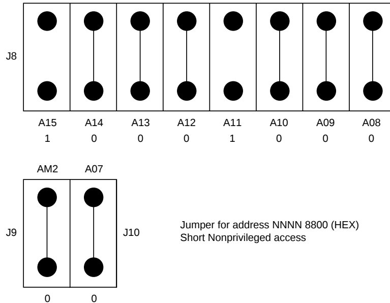
Figure 2-2 Address Jumpers
