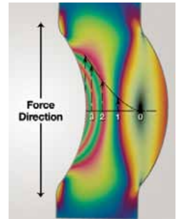
Stress distribution in a C-shaped beam
