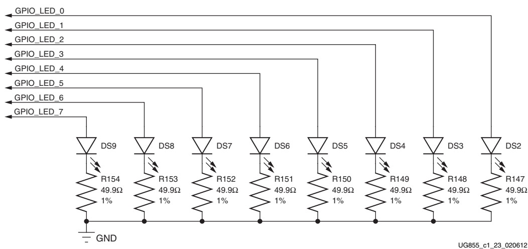
Figure 1-23: User LEDs
