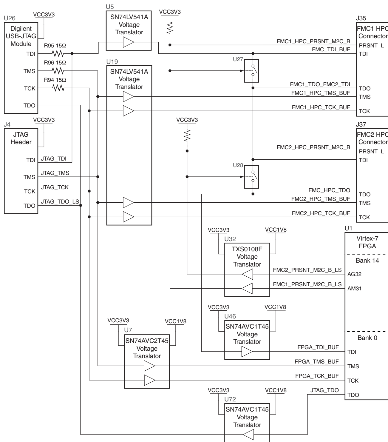
Figure 1-8: JTAG Circuit
