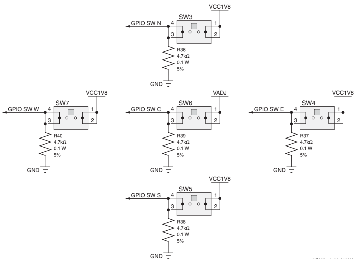
Figure 1-25: User Pushbuttons
