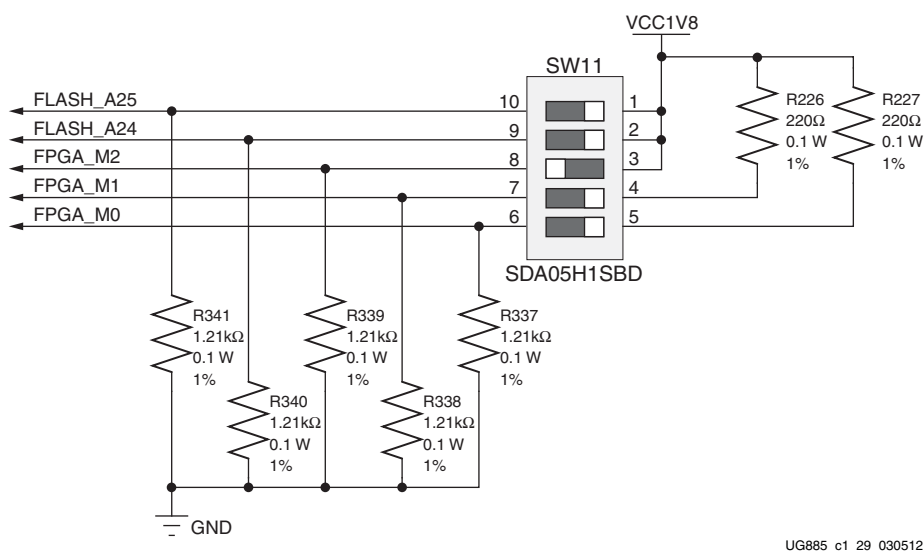
Figure 1-32: Configuration Mode and Upper Linear Flash Address Switch
