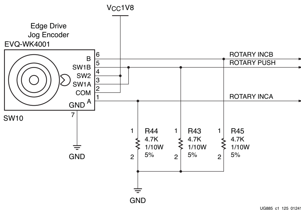
Figure 1-27: User Rotary Switch
