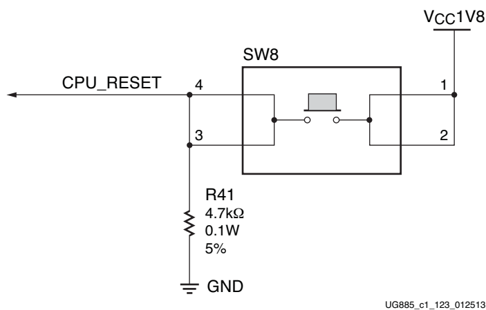
Figure 1-24: CPU Reset Pushbutton
