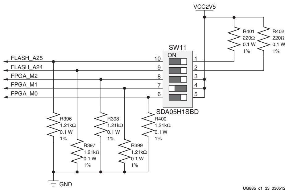
Figure 1-36: Mode Switch
