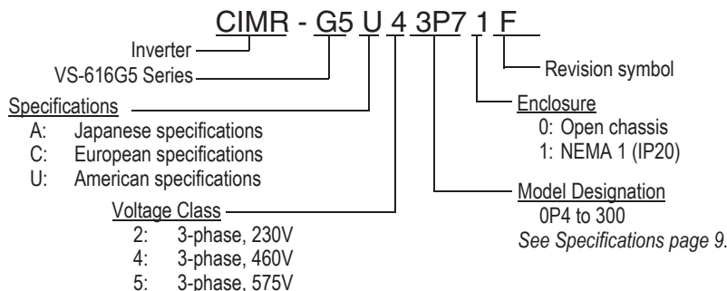
Figure 2 Nameplate Description
