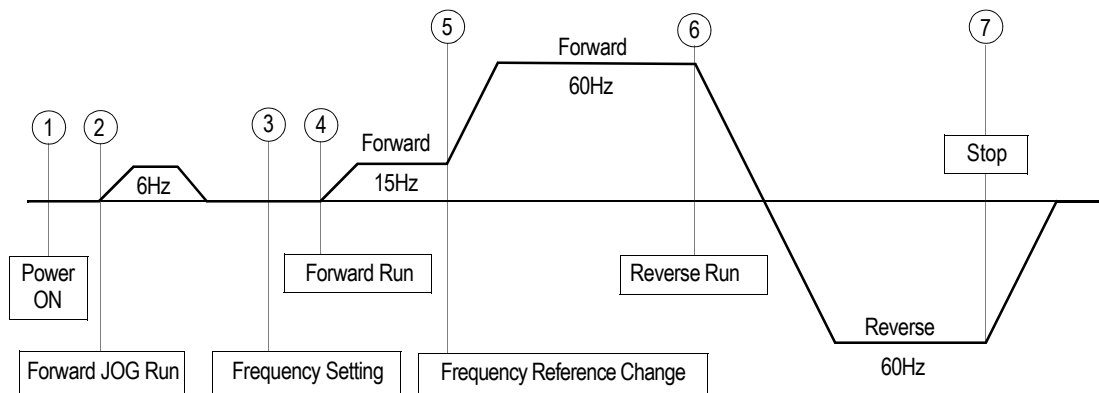
Figure 15 Operation Sequence by Digital Operator
