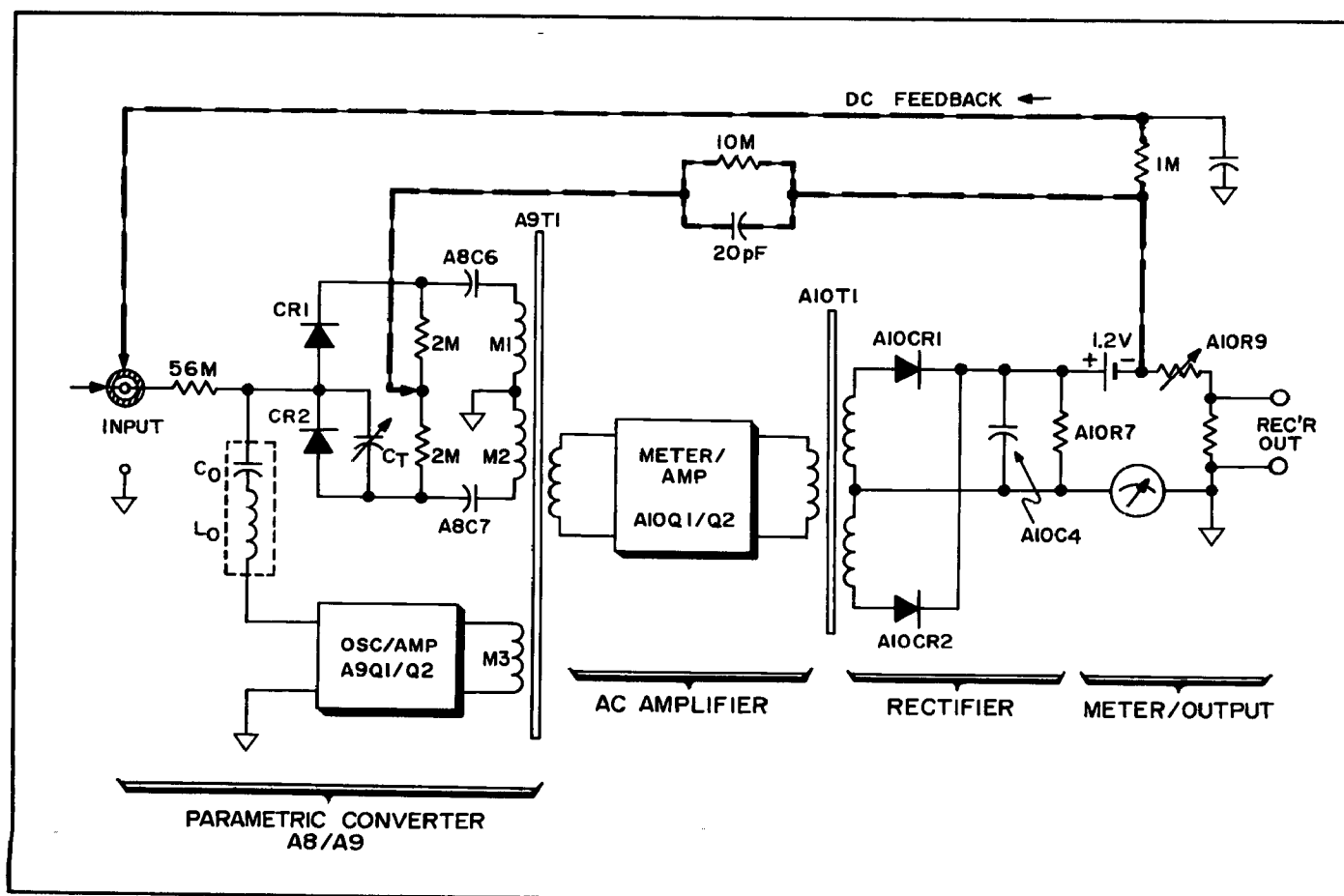
Figure 4-5. Simplified Circuit
