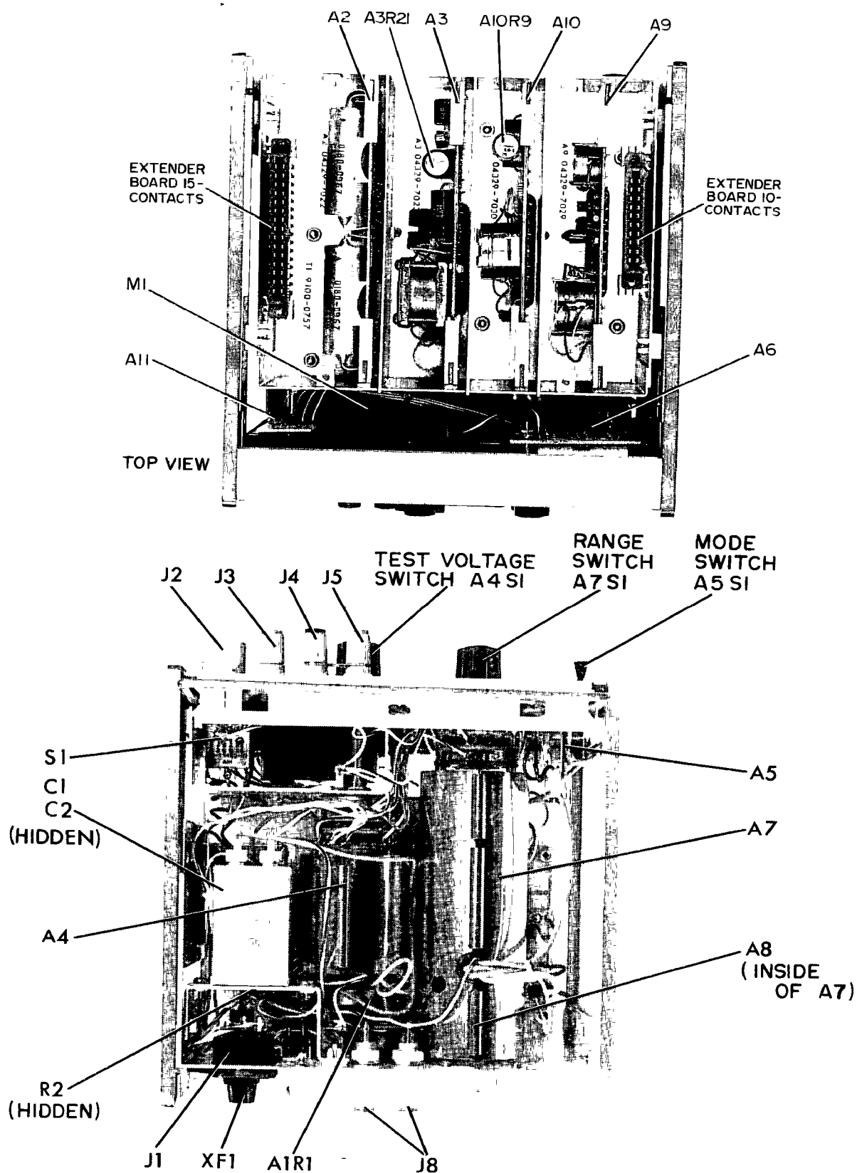
Figure 5-3A. Assembly Location (Top and Bottom View)
