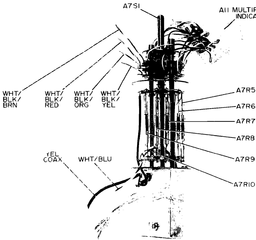
A7 RANGE SWITCH ASS'Y COMPONENT LOCATION
