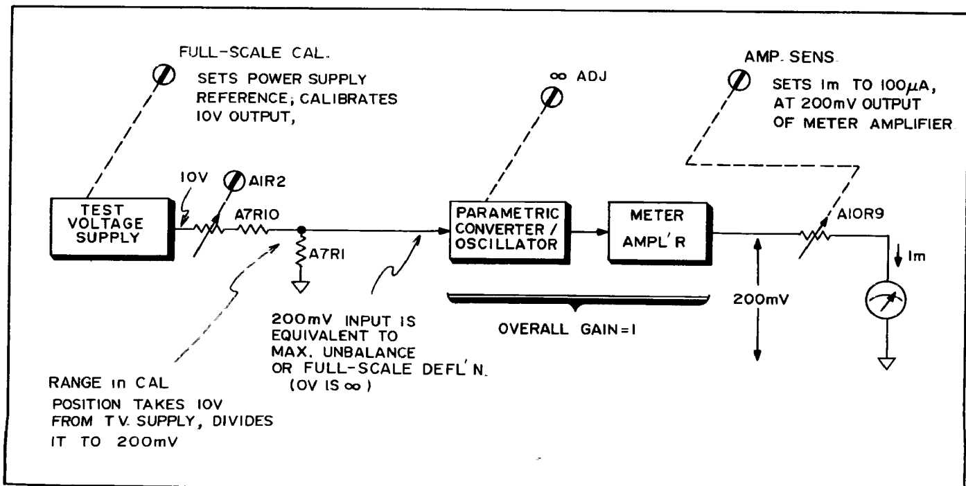
Figure 5-2. 4329A Adjustments
