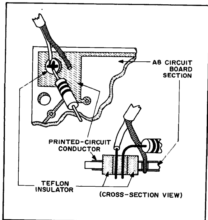
Figure 4-6. Input Insulator Detail
