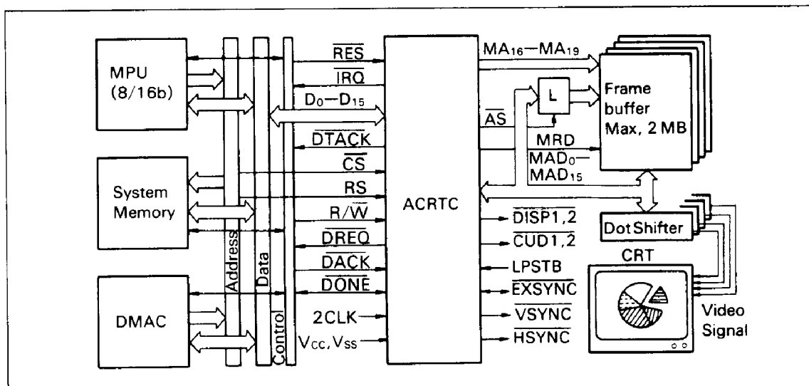
Figure 2 System Configuration
