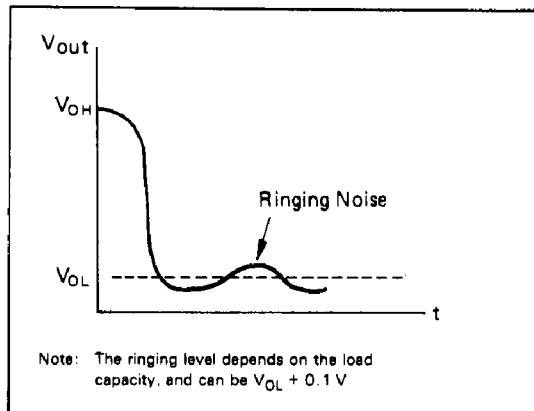
Figure 11. Ringing Noise
