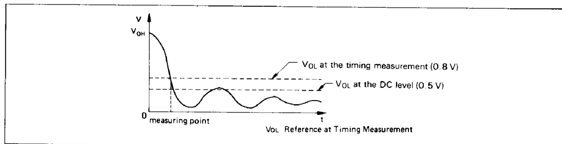
Figure 16. Test Points
