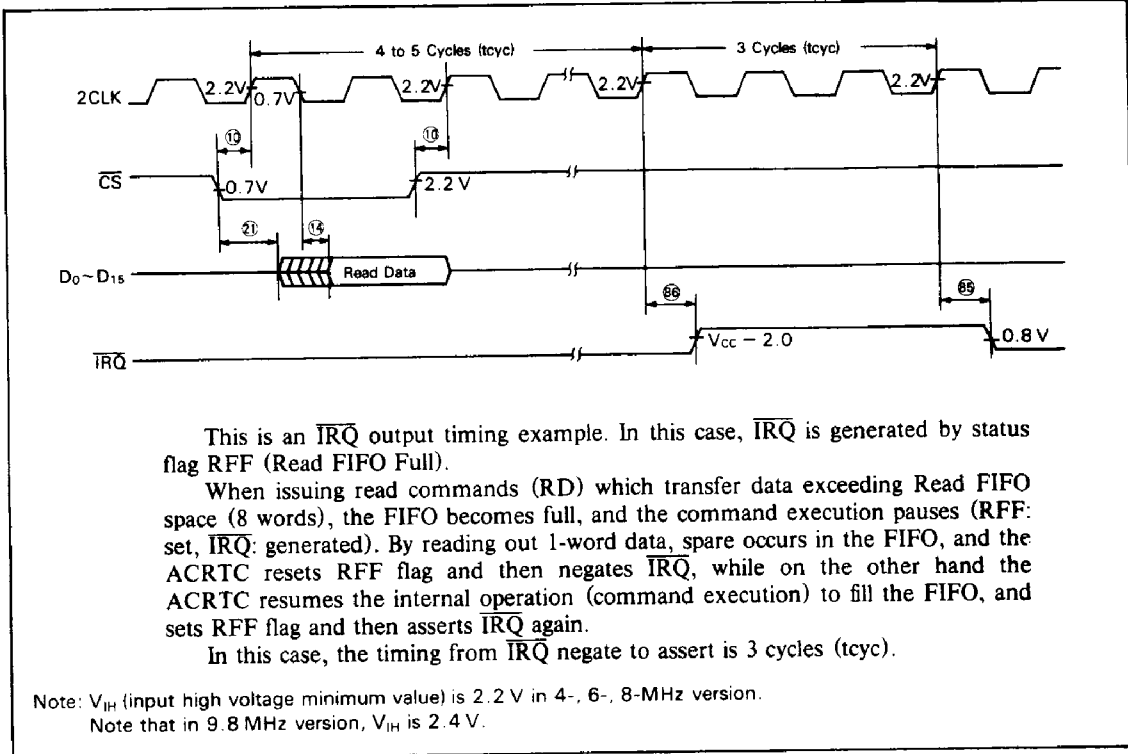
Figure 35. IRQ Output Timing (Example: Read FIFO Full Interrupt Enable)
