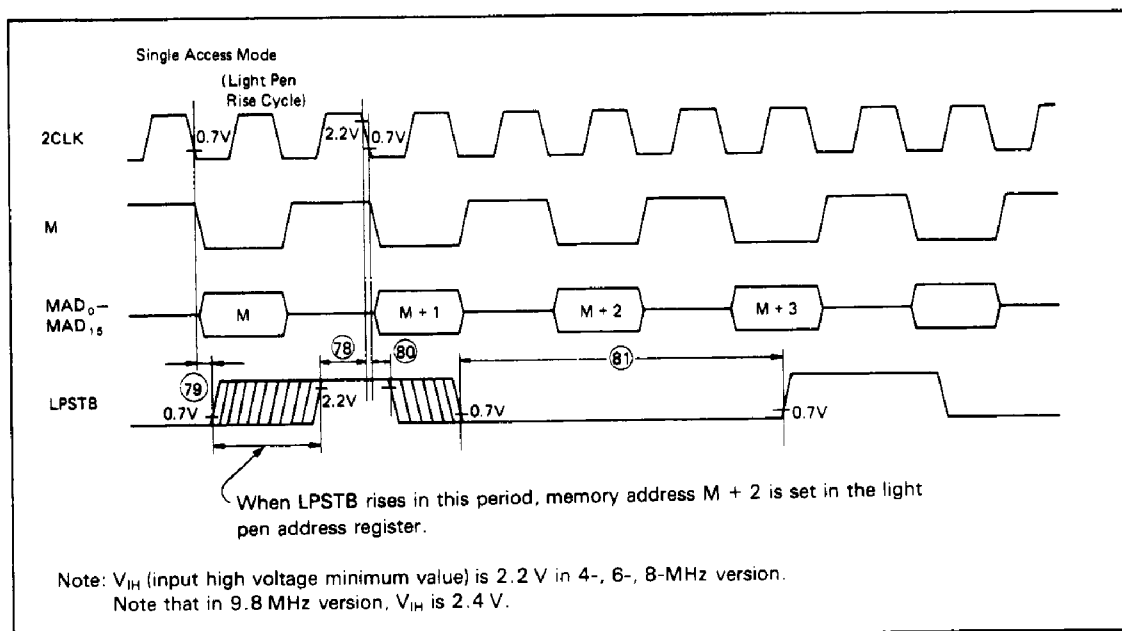
Figure 31. LPSTB Input Timing (Single Access Mode)
