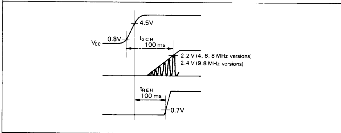
Figure 10. Power-On Sequence
