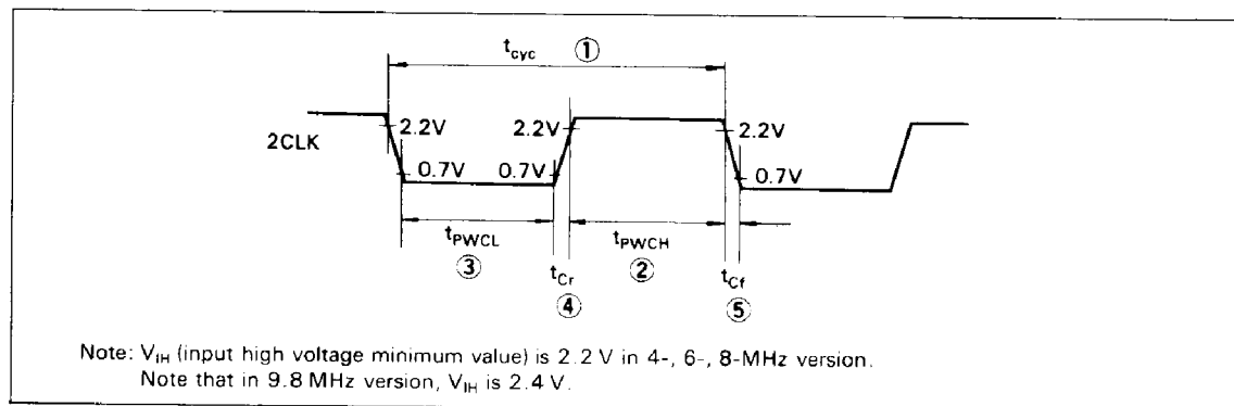
Figure 17. 2CLK Waveform
