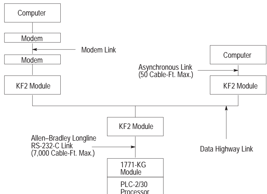
Figure 1.2 Point-to-Point Links
