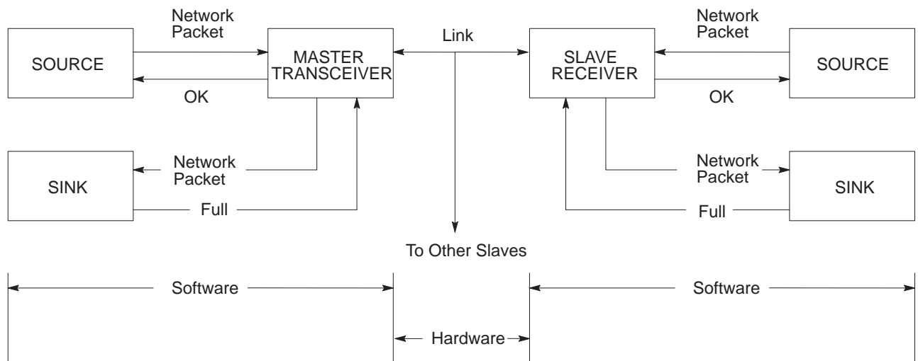
Figure 4.15 Slave Transceiver
