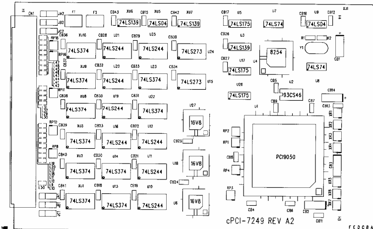
Figure 2.3.4 cPCI-7249R Layout
