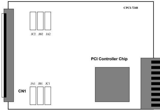
Figure 2.3.3 cPCI-7248 PCB Layout
