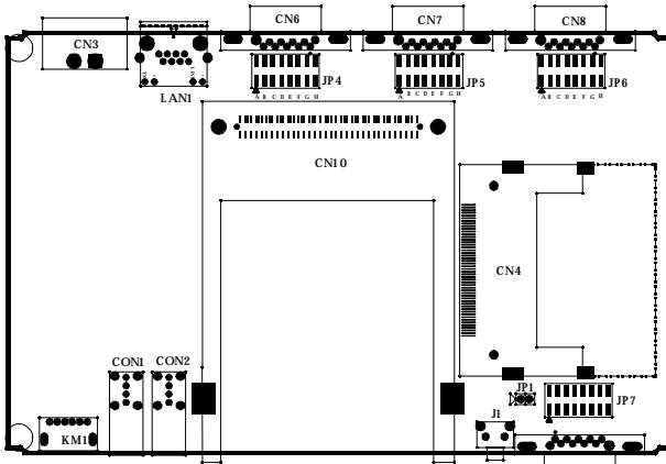
Figure A-1: WebLink-2059 connector and jumper locations (Top View)
