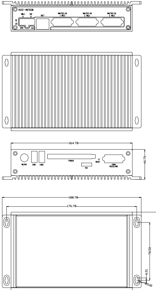
Figure 1-1: Chassis dimensions
