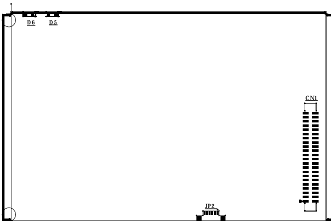
Figure A-2: WebLink-2059 connector and jumper locations (Bottom View)
