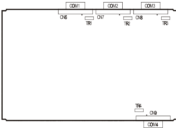
Figure A-3: COM ports terminator resistor locations
