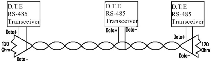
Figure A-5: RS-485 Wiring topology
