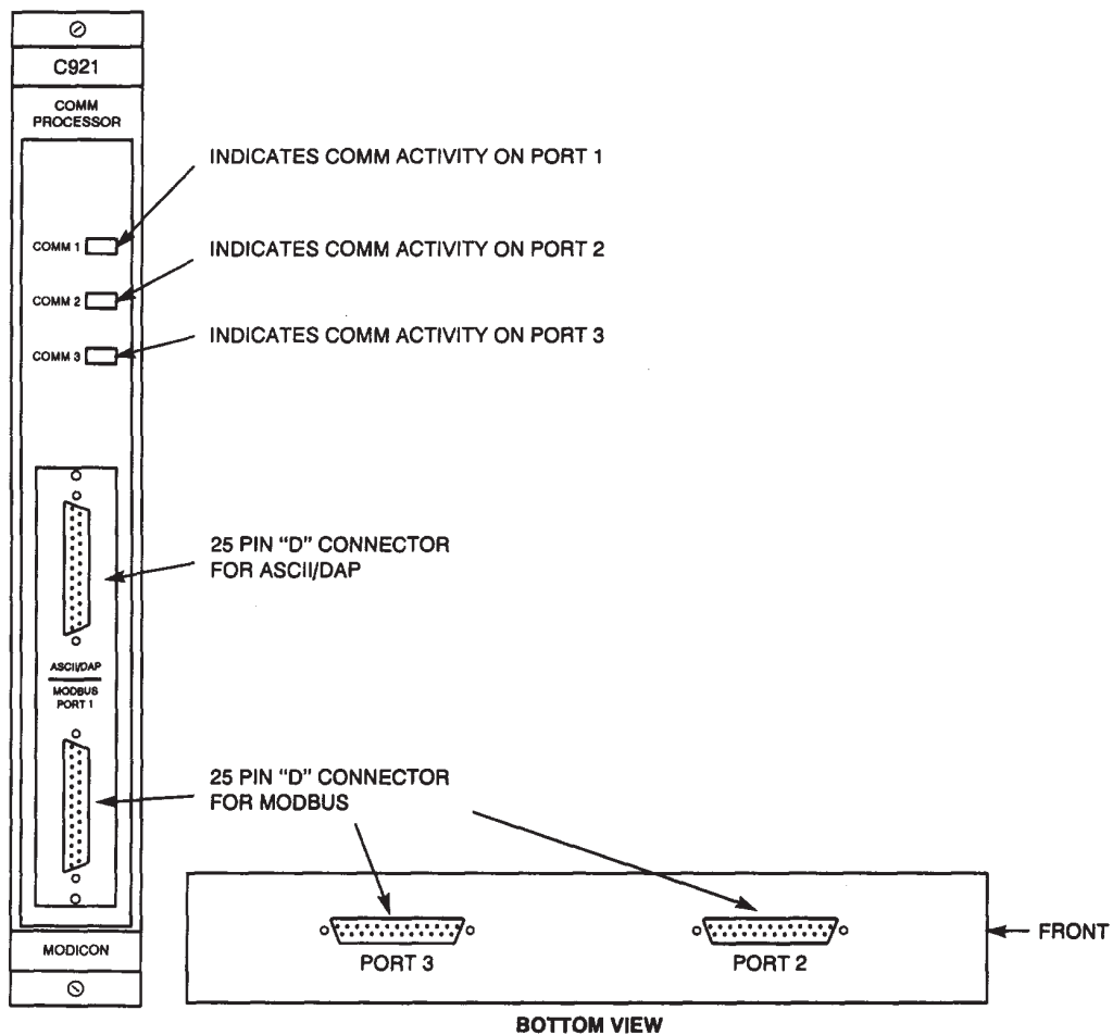
Figure 2-35 C921-100 Communications Processor Module
