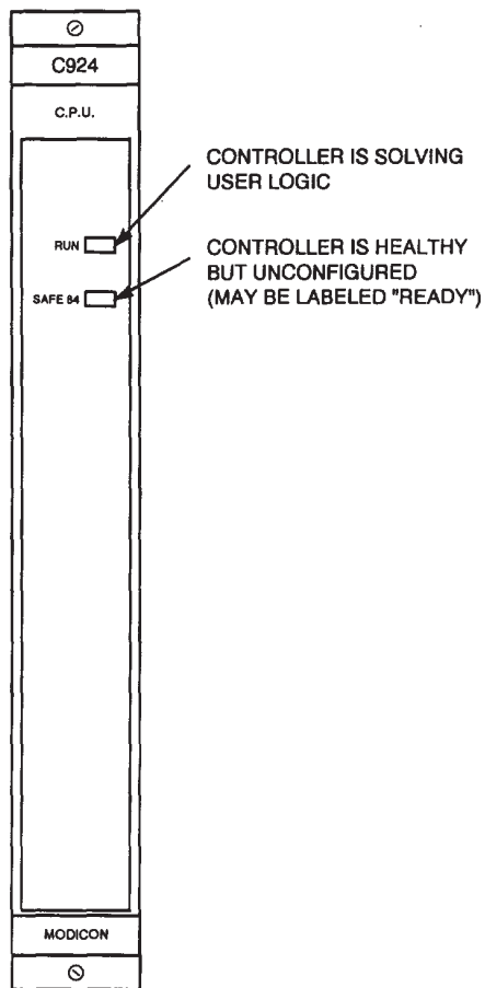
Figure 2-38 C924-000 Central Processing Unit (CPU) Module
