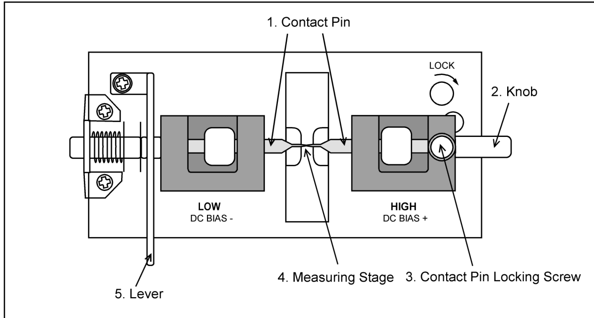
Figure 1-2 16034H Parts
